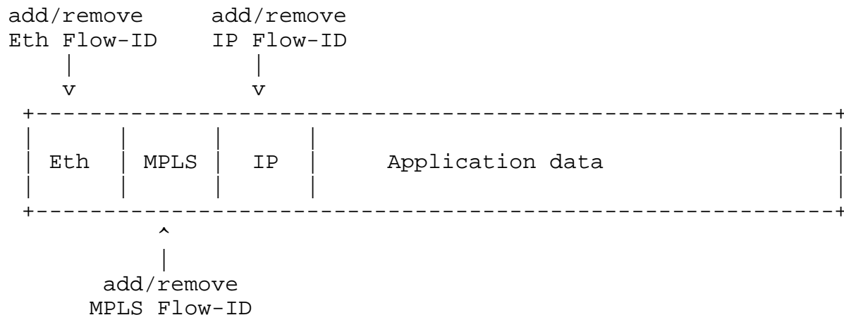
Figure 9: Packet with multiple Flow-IDs
