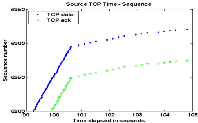
TCP SACK: WLAN->GPRS src TCP
