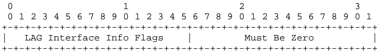
Figure 4: LAG Interface Info TLV
