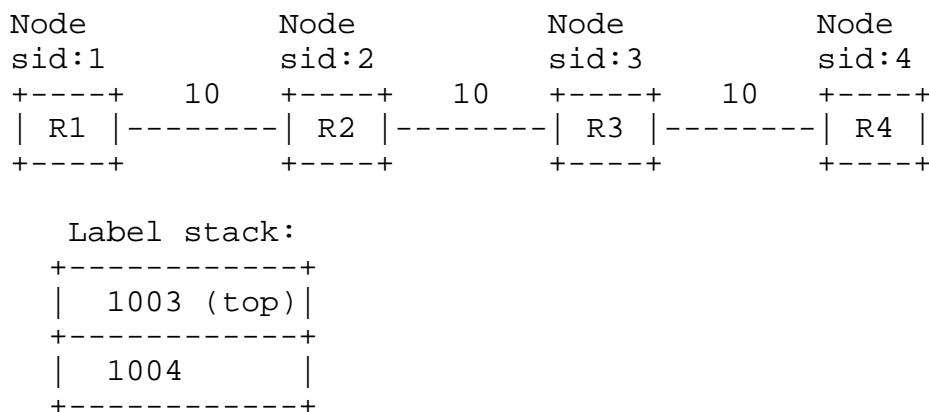
Figure 1: Example topology with SRGB 1000-2000
