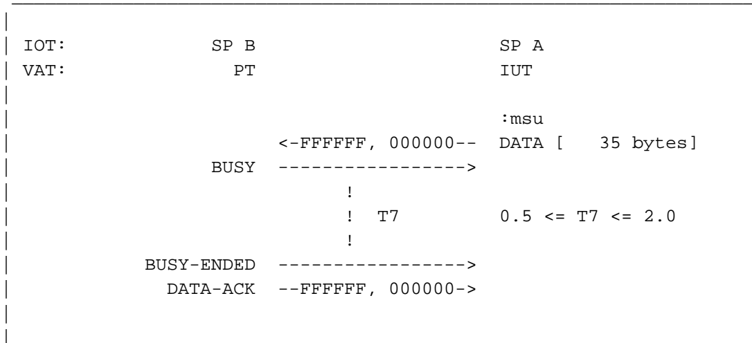
Figure 3.10.2-1. Timer T7
