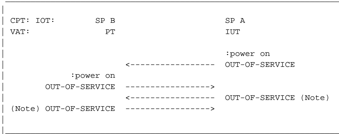
Figure 3.1.1-2. Initialization (Power-up)
