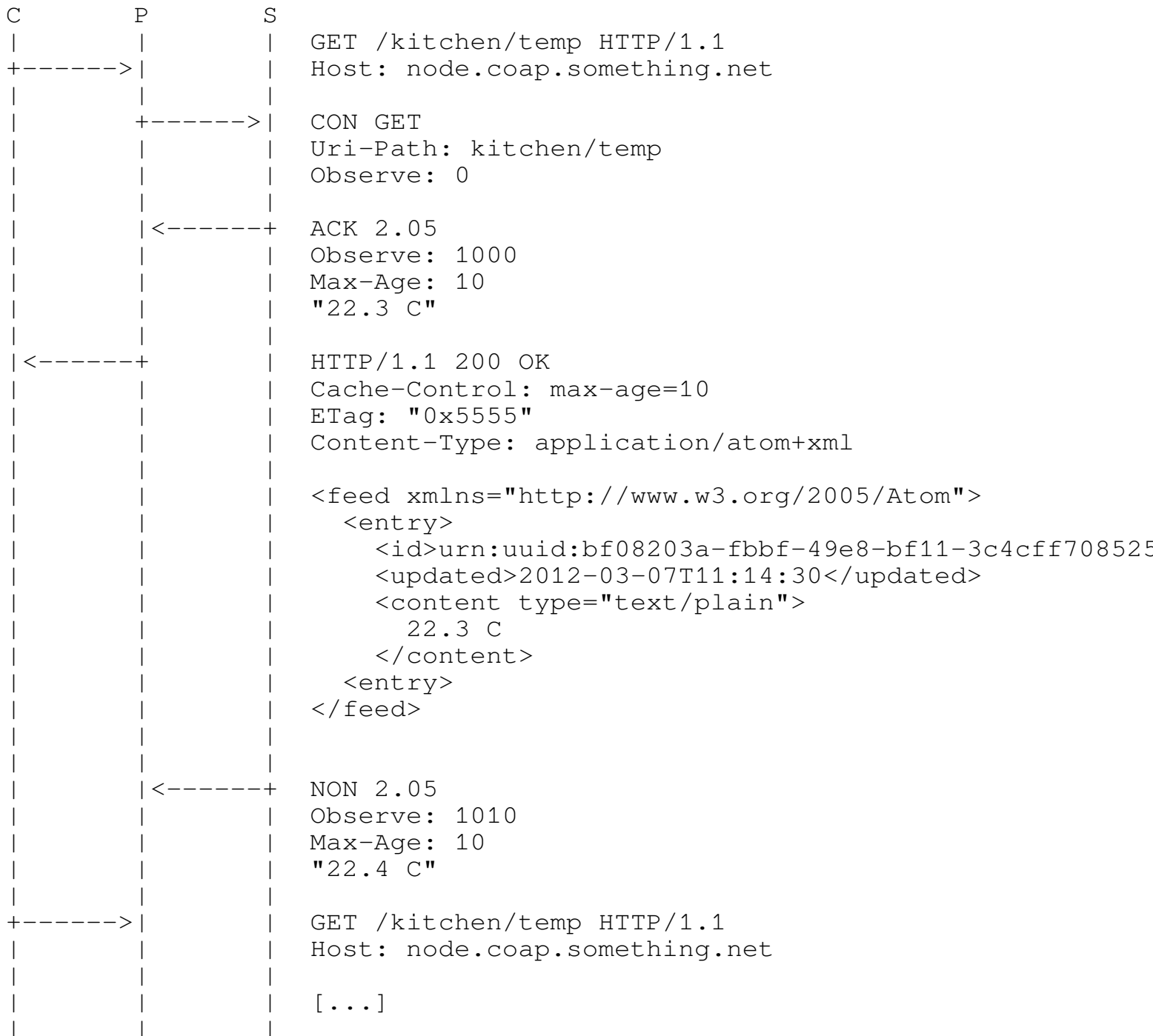
Figure 7: Observation via Atom feeds
