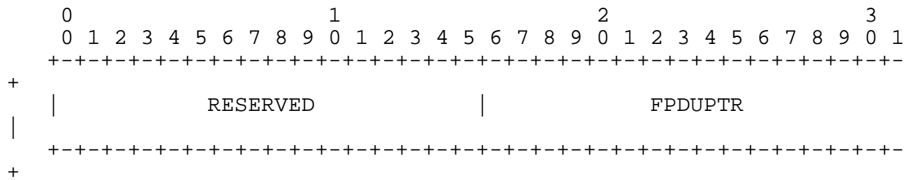
Figure 3 Marker Format
