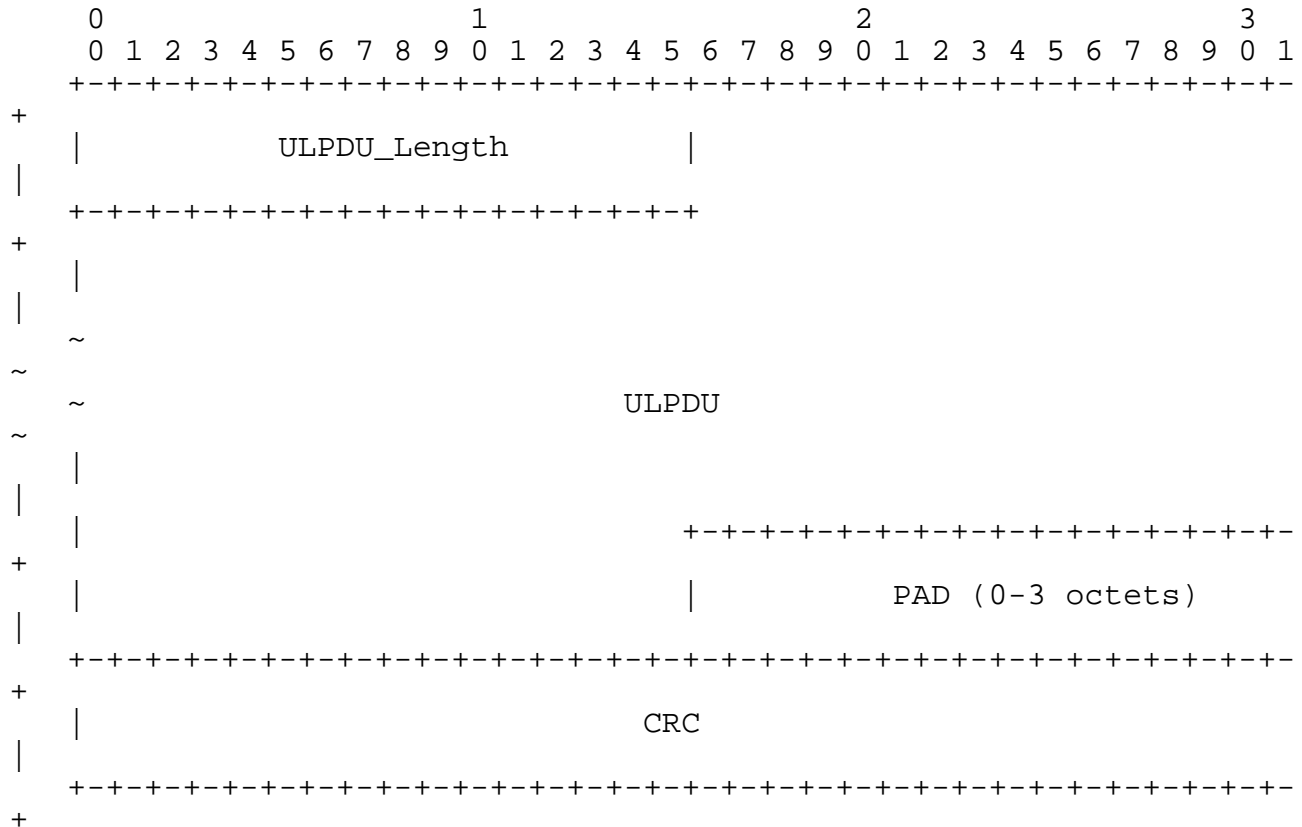
Figure 2 FPDU Format
