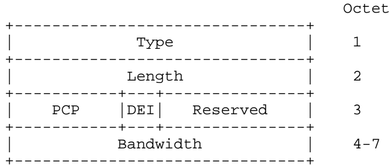
Figure 5: Bandwidth Assignment sub-TLV
