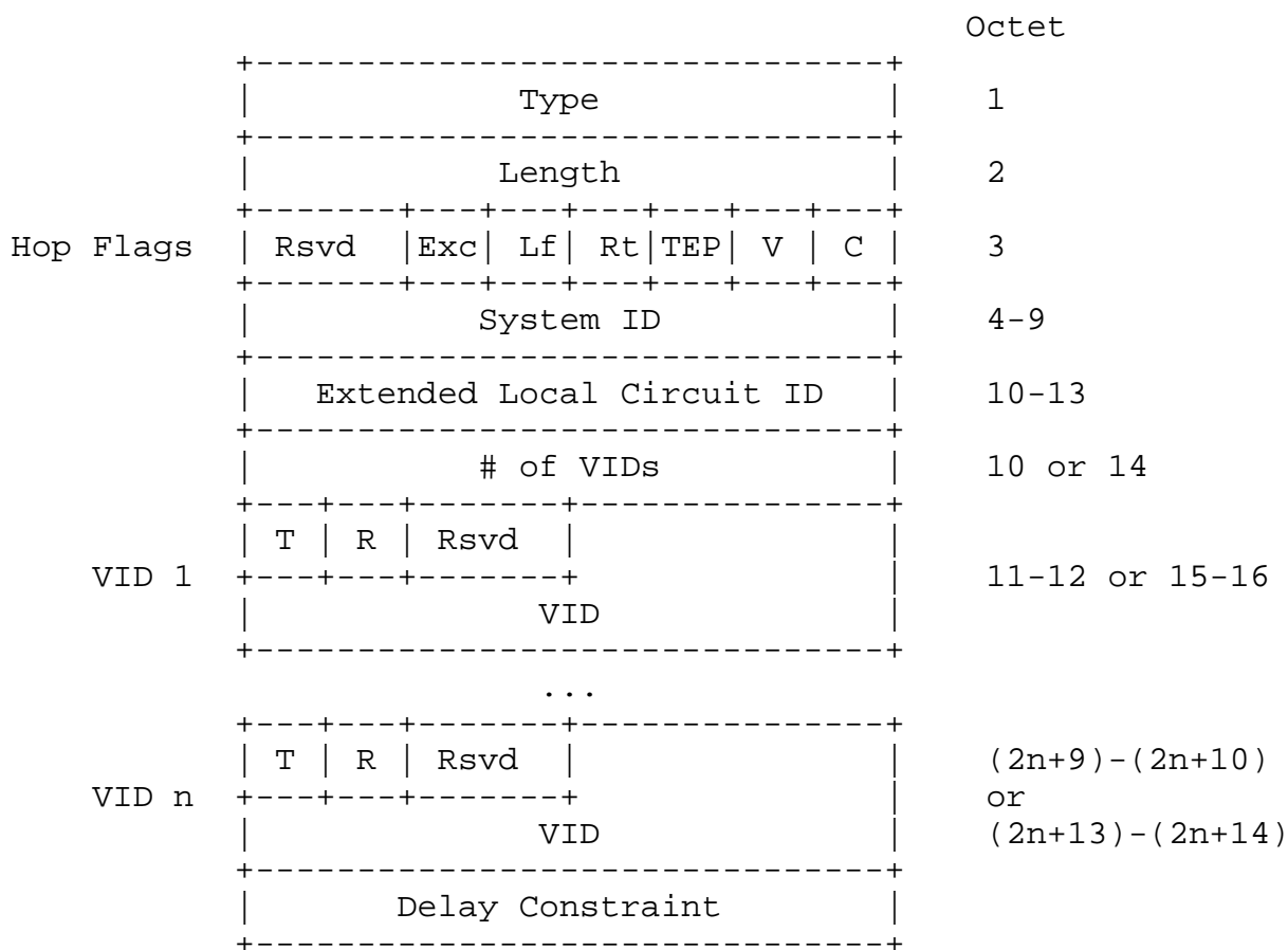
Figure 3: Hop sub-TLV
