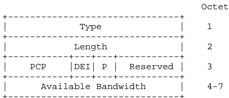
Figure 4: Bandwidth Constraint sub-TLV
