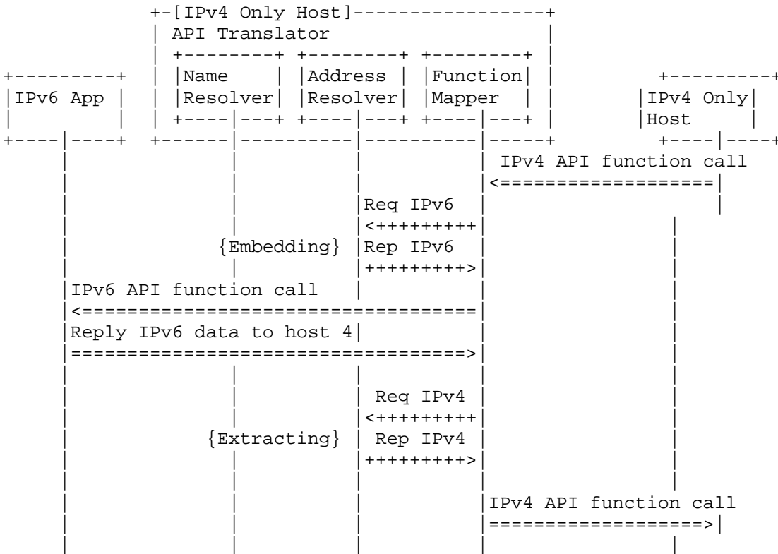
Figure 8: Behavior of receiving data from IPv4 host
