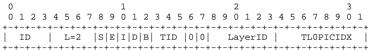
Long Frame Marking RTP Extension for [VVC]
