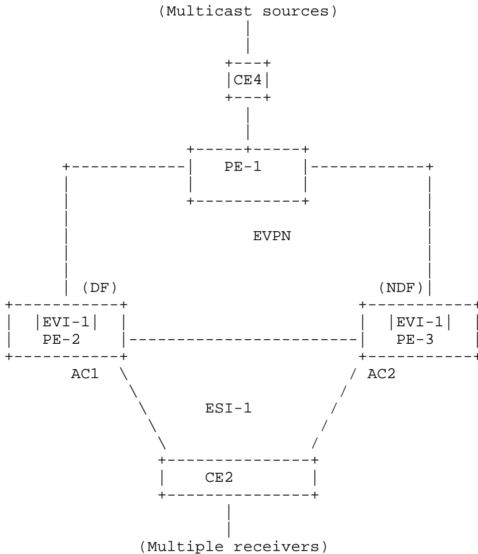
Figure 1: Multi-homing Network of EVPN for IPTV deployments
