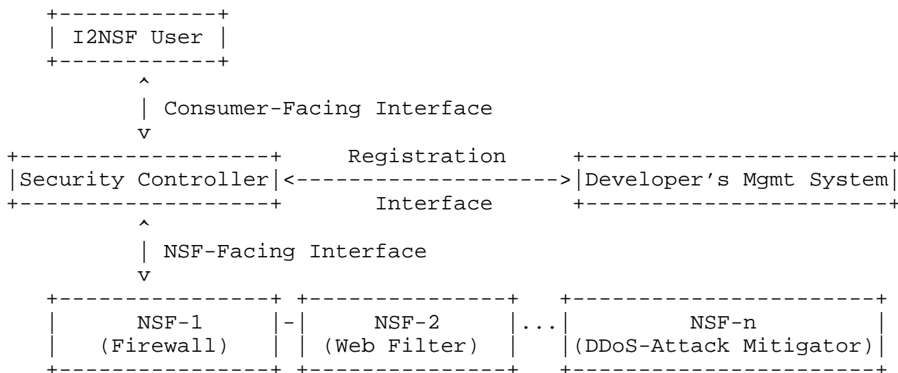
Figure 1: I2NSF Framework
