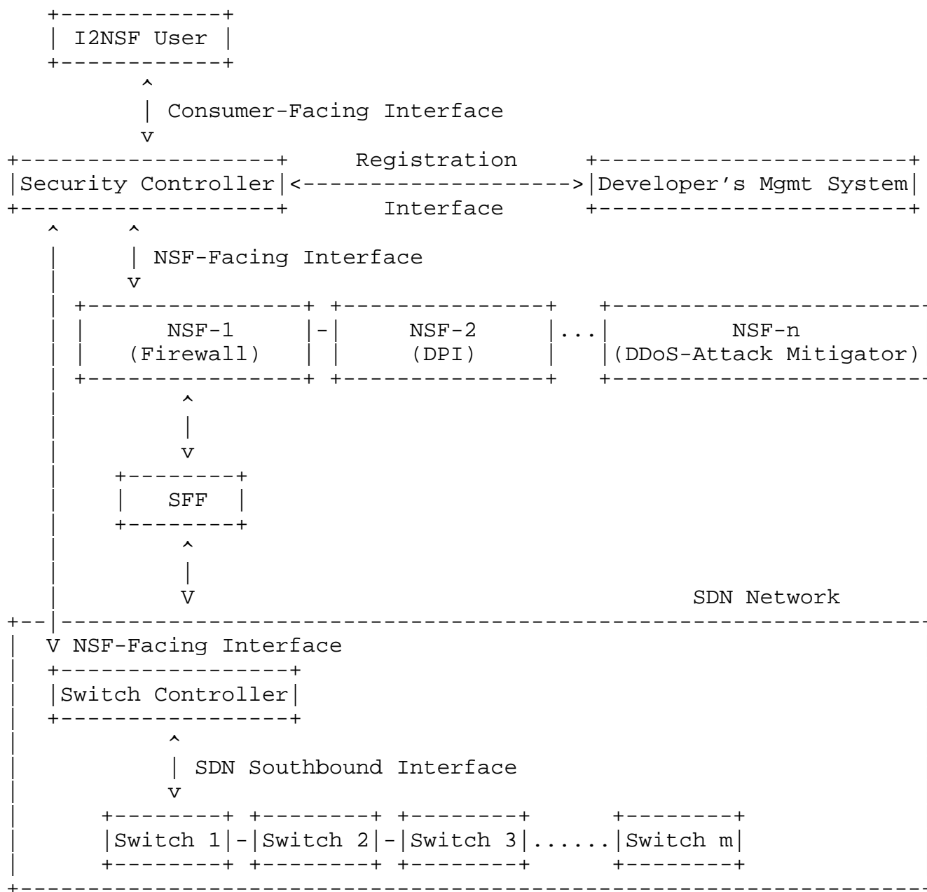
Figure 2: An I2NSF Framework with SDN Network
