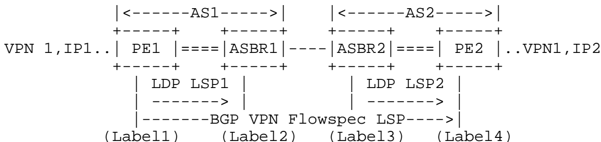
Figure 1: Usage of FlowSpec with Label
