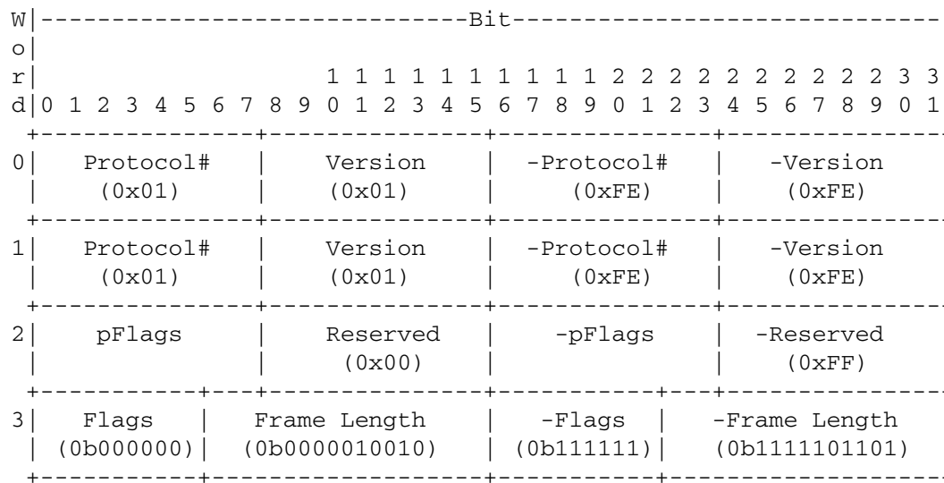
Fig. 9 FSF Format (part 1 of 2)
