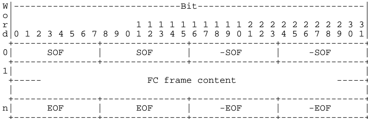
Figure 16 -- FC Frame Encapsulation Format
