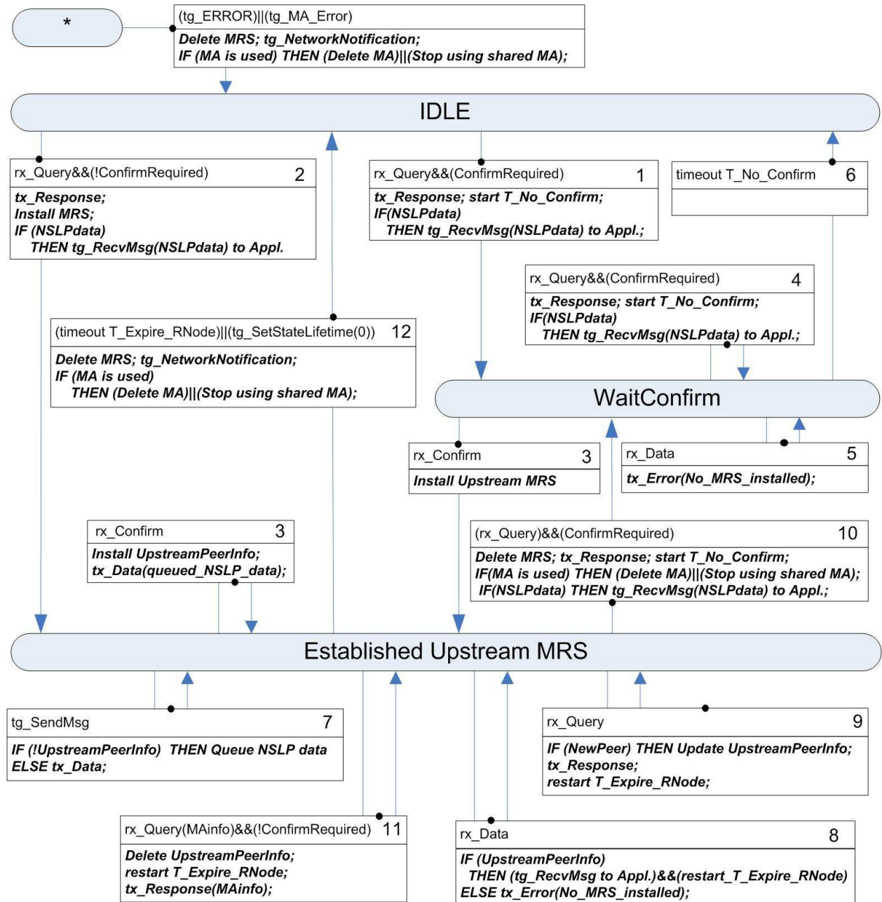
Figure 3: GIST Responding Node State Machine
