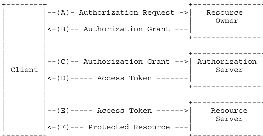
Figure 1: Abstract OAuth 2.0 Protocol Flow
