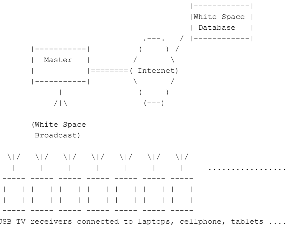
Figure 6: White Space Used for Local TV Broadcast
