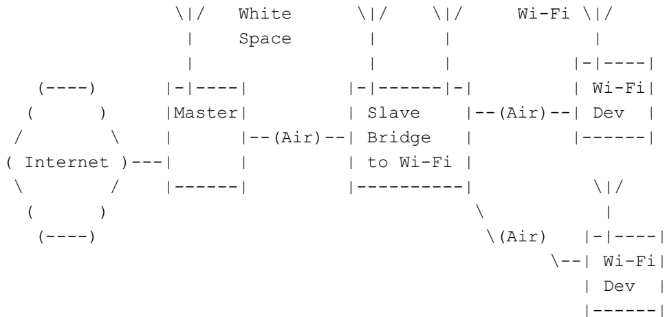
Figure 4: White Space Network Used for Backhaul
