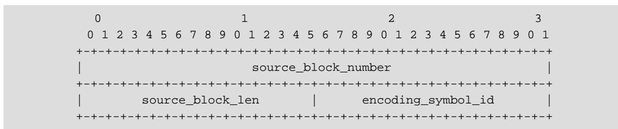
Figure 5: Example: FEC Payload Id Format for 'fec_id' = 129
