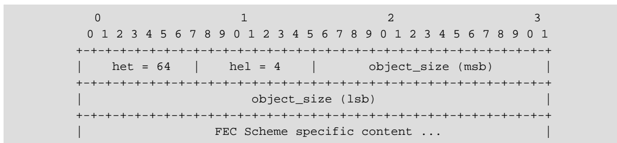
Figure 6: EXT_FTI Header Extension General Portion Format
