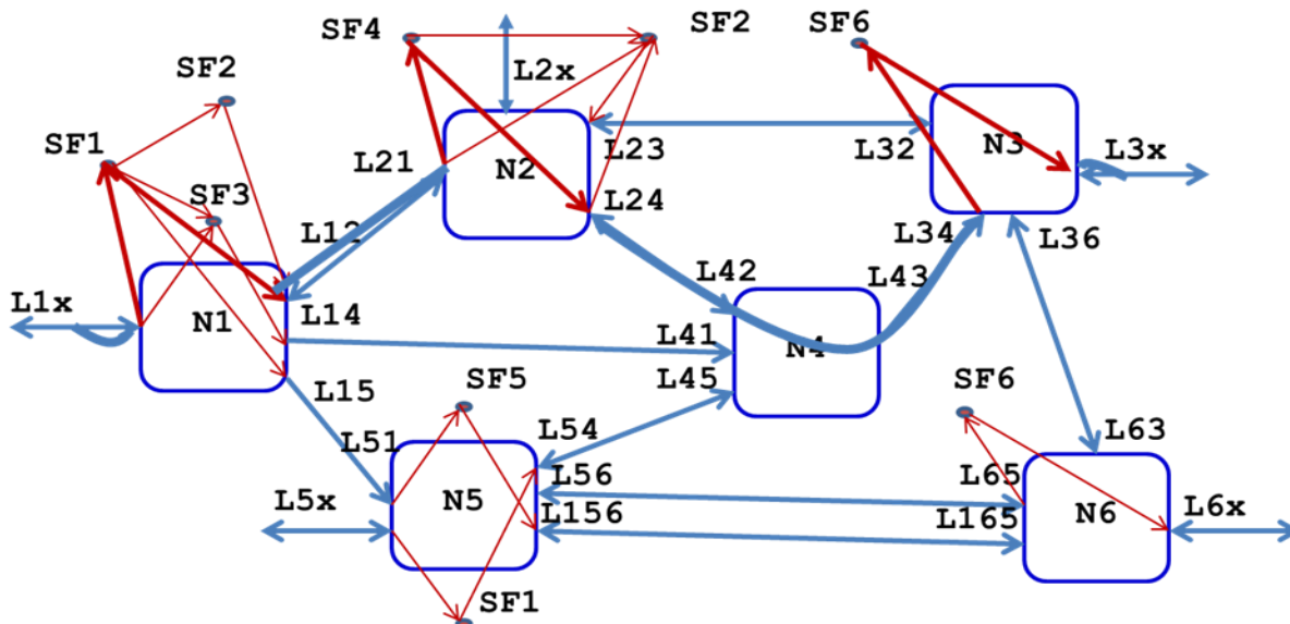
Figure 3: SFC with TE constraints
