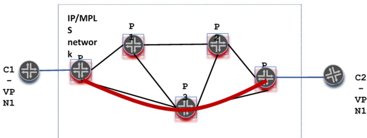
Figure 2: L3 VPN with delay constraints
