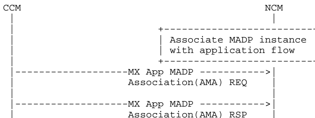
Figure 9: MAMS Application MADP Association Procedure
