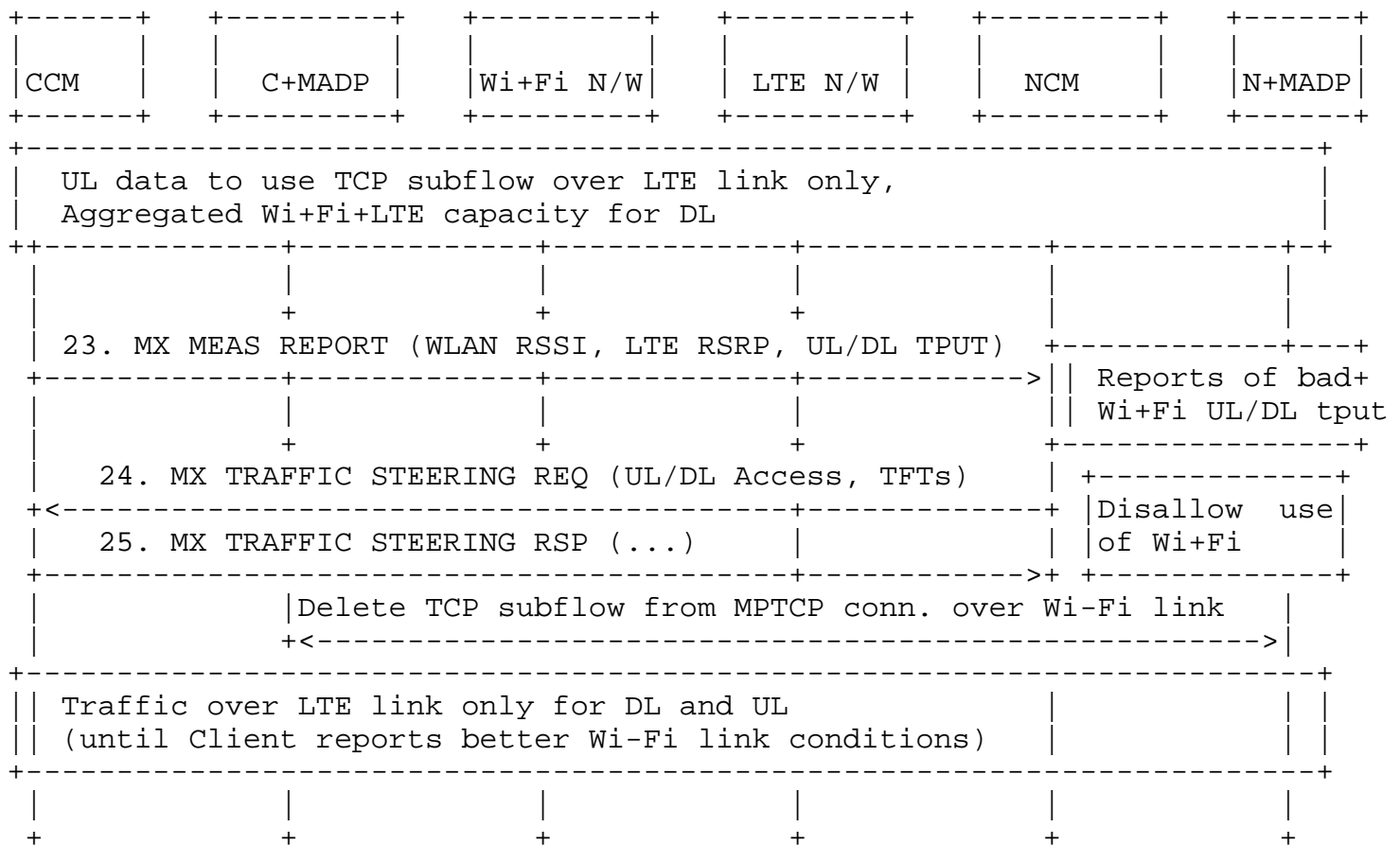
Figure 18: MAMS-assisted MPTCP Proxy as User Plane - Part 4
