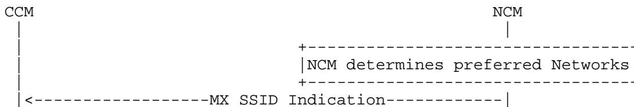
Figure 10: MAMS Network ID Indication Procedure
