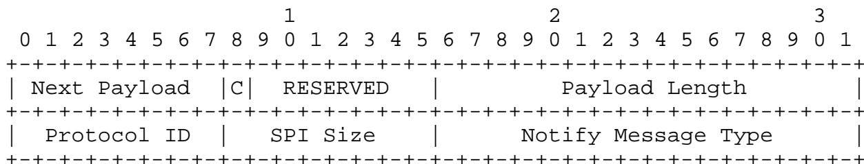
Figure 7: Notify Payload
