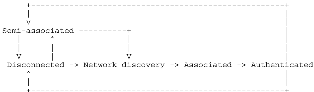
Node-F connectivity state machine.
