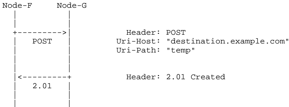
Sending a message in a semi-associated state.
