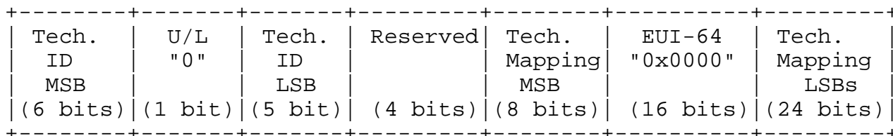
Figure 1: general format of the host ID part for legacy protocols
