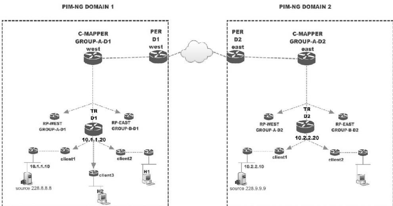
Figure 46 network with 2 multicast domains
