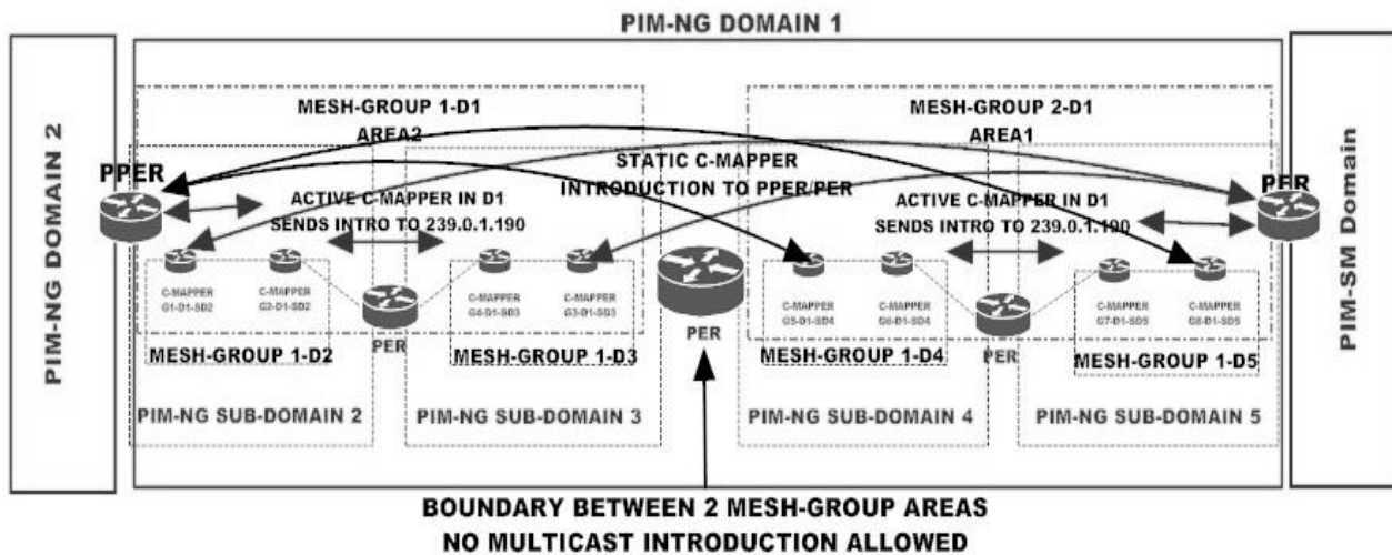
Figure 53 PPER and PER communication with C-MAPPER
