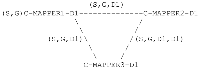
Figure 45 Intra-Domain connectivity and RPF check
