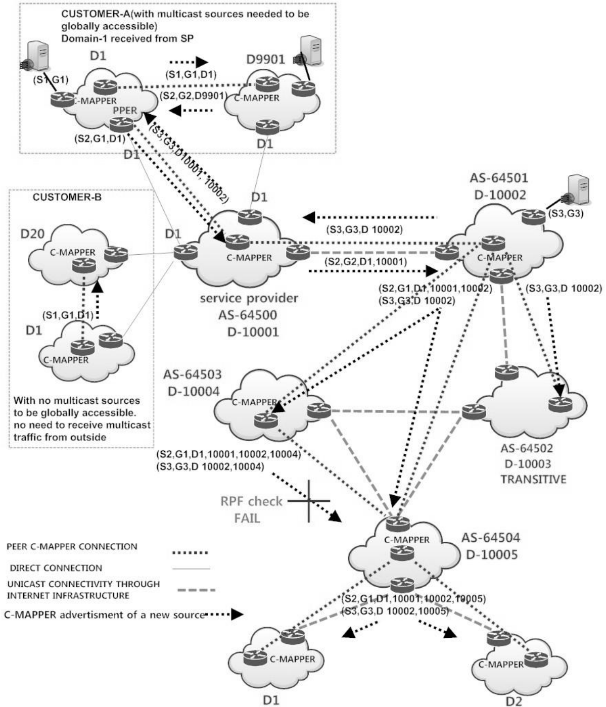
Figure 51 multicast network and multicast advertisements
