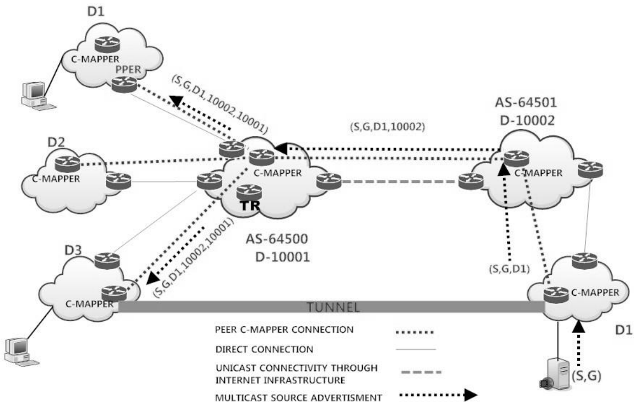
Figure 48 core domain implementation
