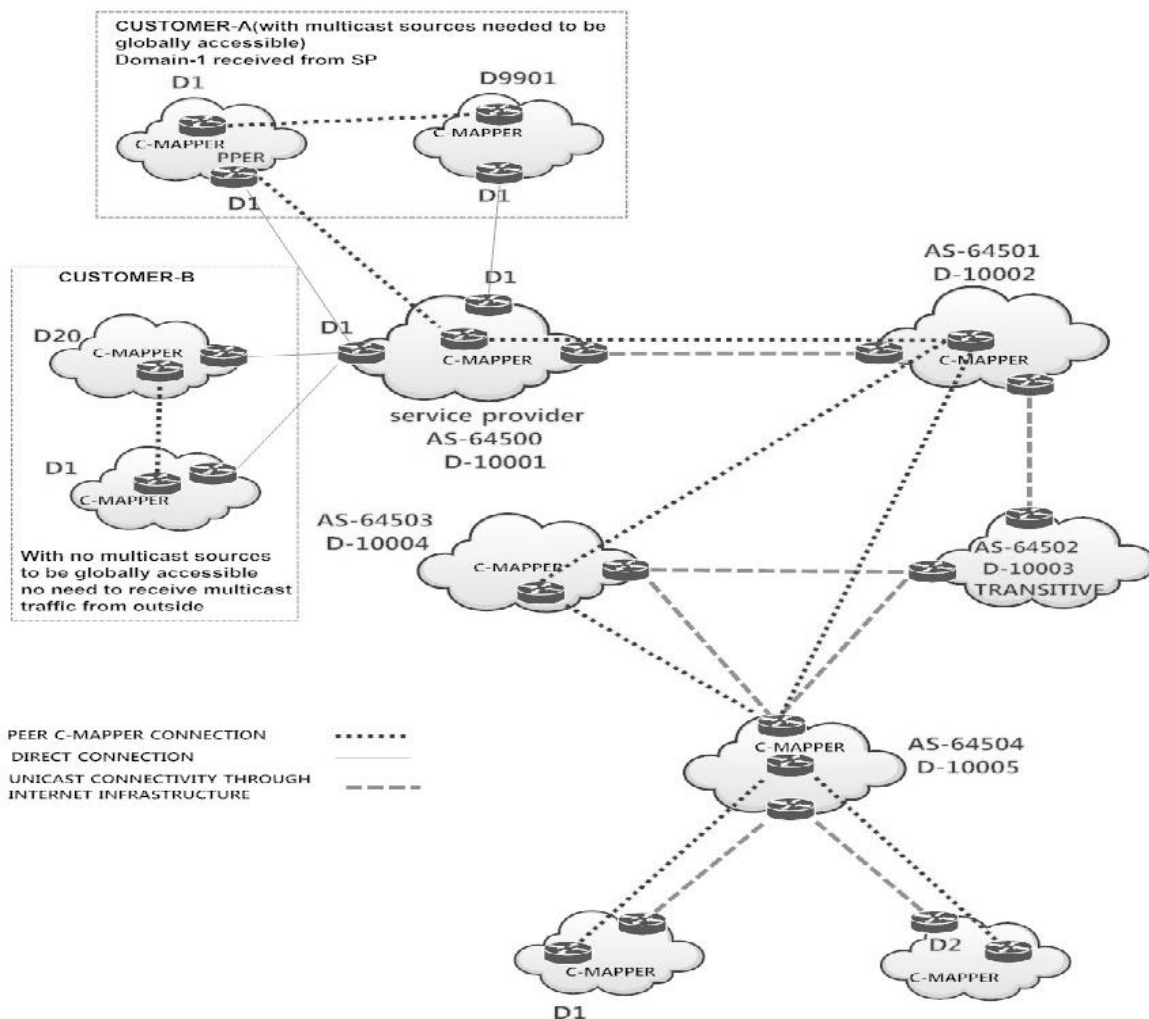
Figure 50 network with multiple multicast domains
