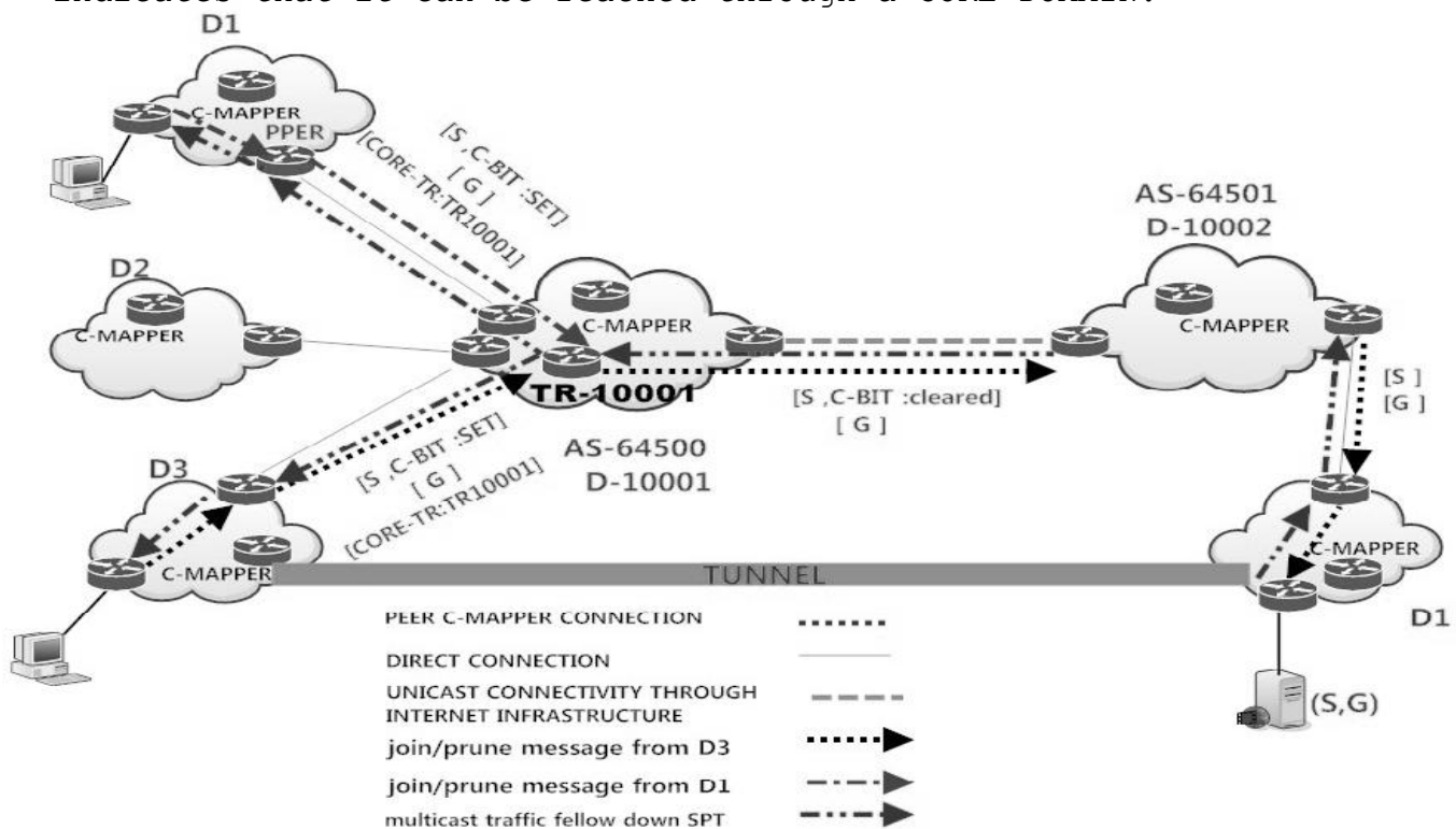
Figure 49 join/prune message being sent towards the source
