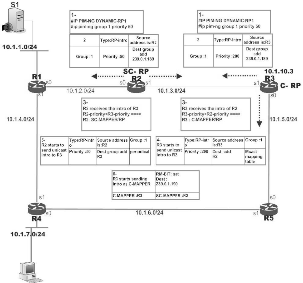
Figure 20 PIM-NG network with backup RP (SC-RP)
