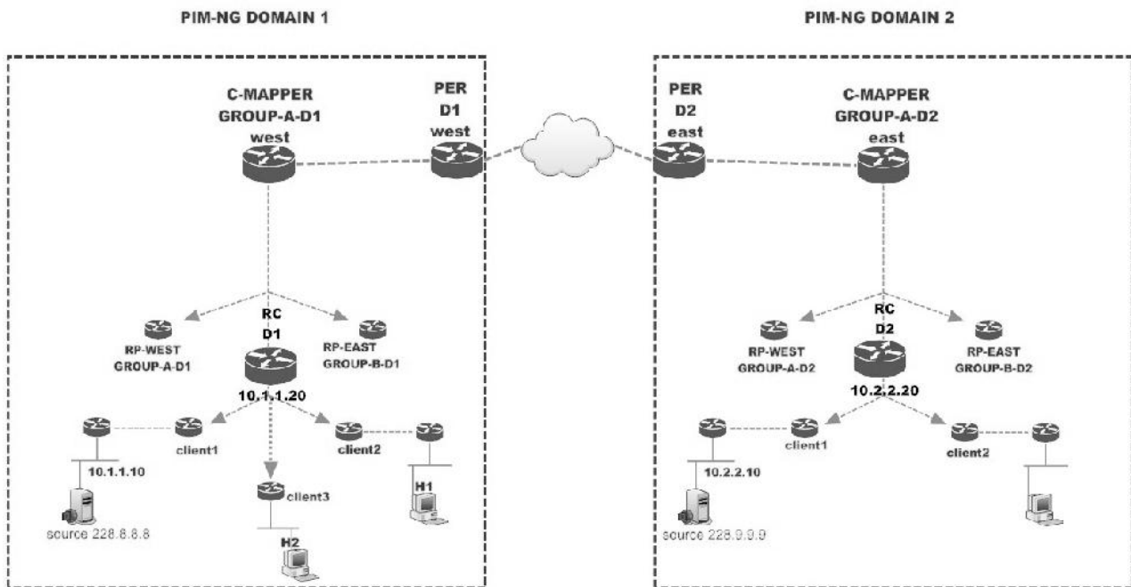
Figure 39 network with 2 PIM-NG multicast domains
