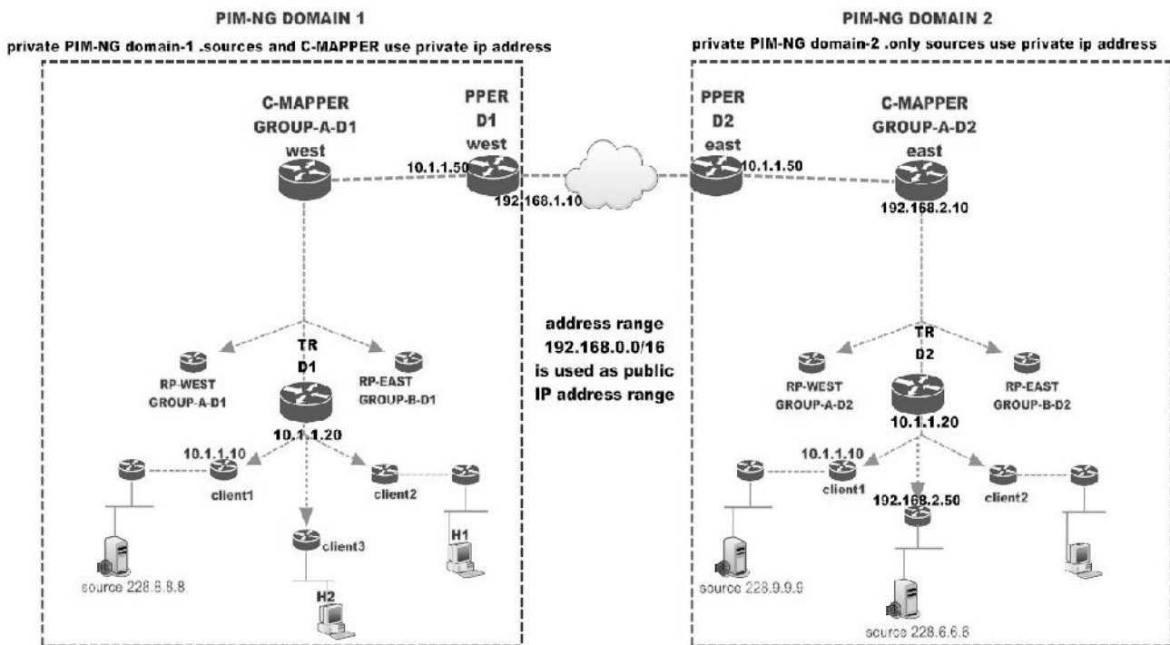
Figure 47 Multicast network with private PIM-NG domains
