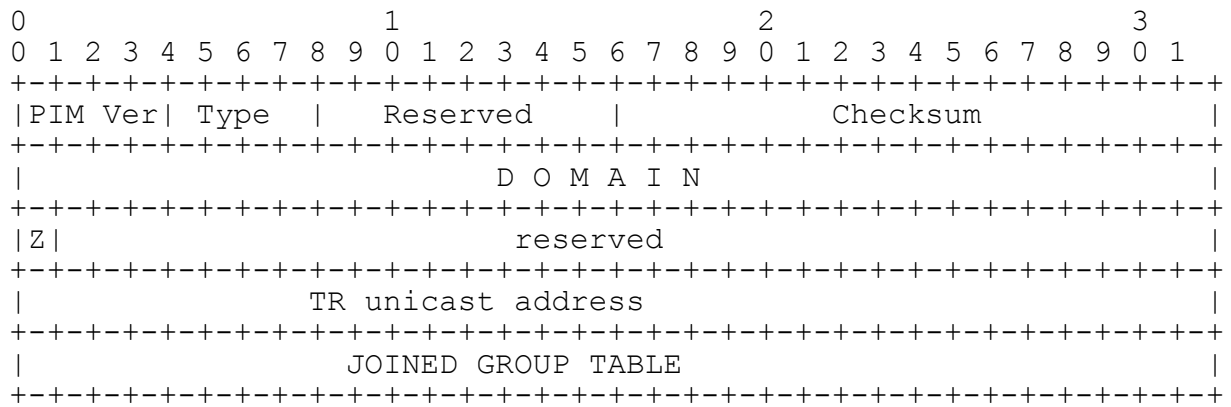
Figure 42 TR introduction message
