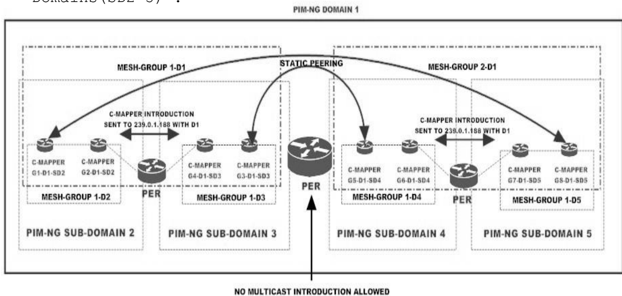
Figure 52 Mesh-Groups and C-MAPPER peering
