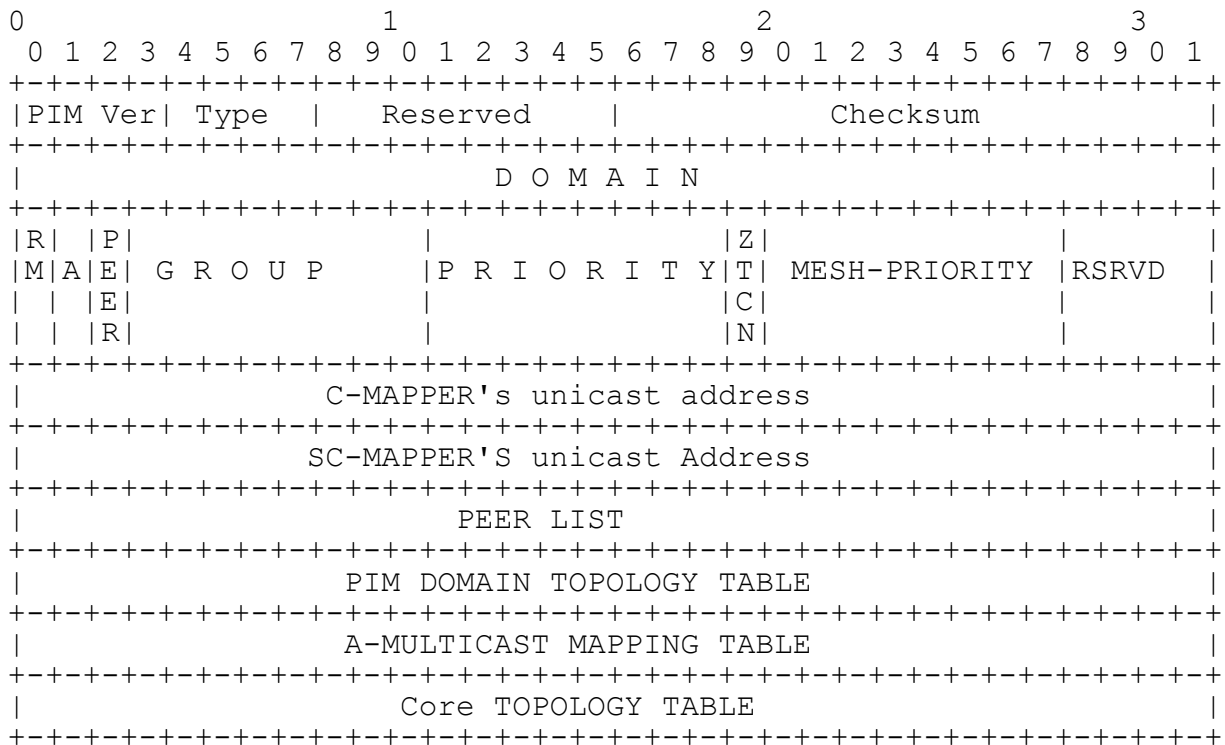
Figure 36 introduction message format sent to ALL PIM-NG MAPPERS 224.0.1.188
