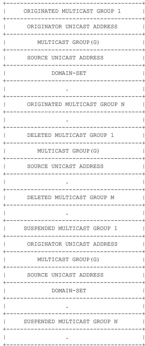
Figure 32 AMMT Format
