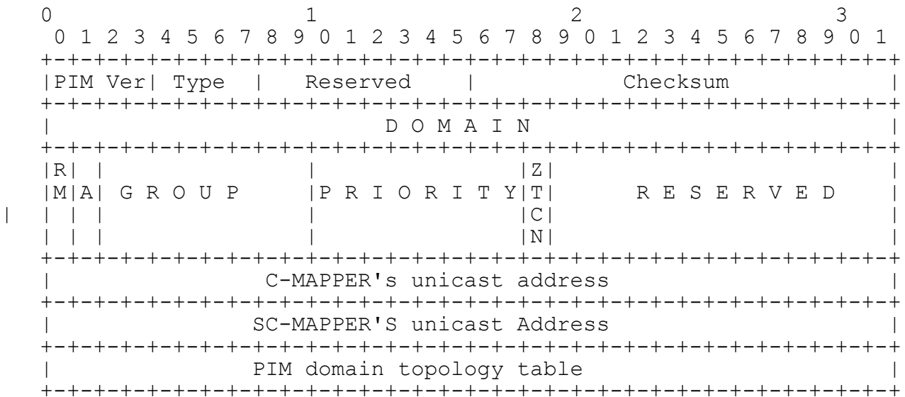
Figure 18 SC-MAPPER/RP answers to a host REQUEST-FOR-C-MAPPER message
