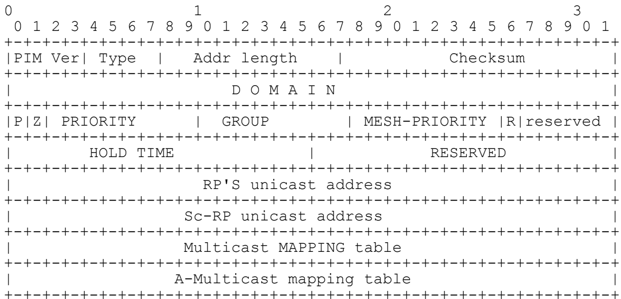
Figure 21 RP introduction message format
