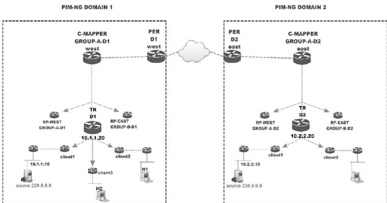
Figure 45 network with 2 multicast domains
