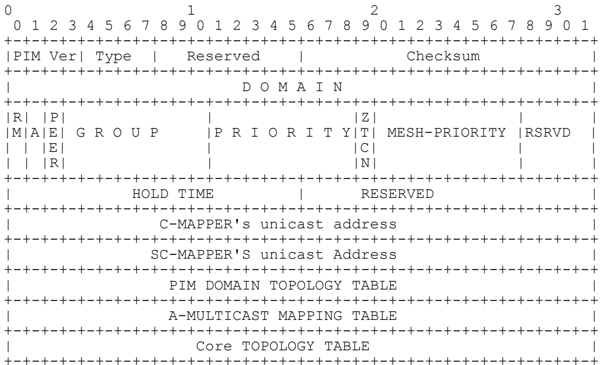
Figure 35 introduction message format sent to ALL PIM-NG MAPPERS 224.0.1.188
