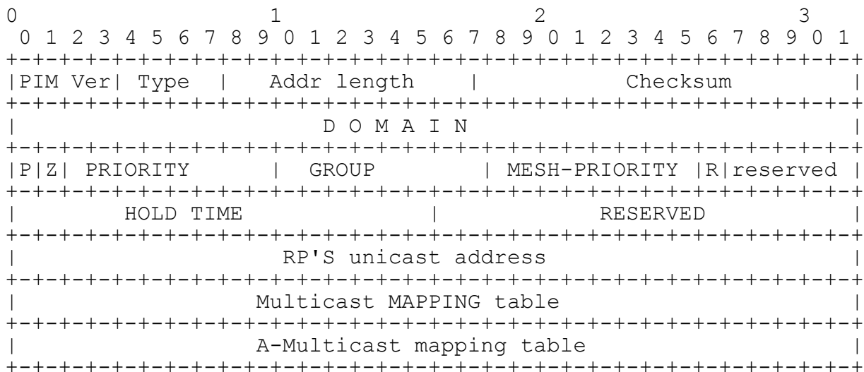
Figure 22 C-MAPPER/RP unicast HELLO/KEEP-ALIVE message to back up RPs
