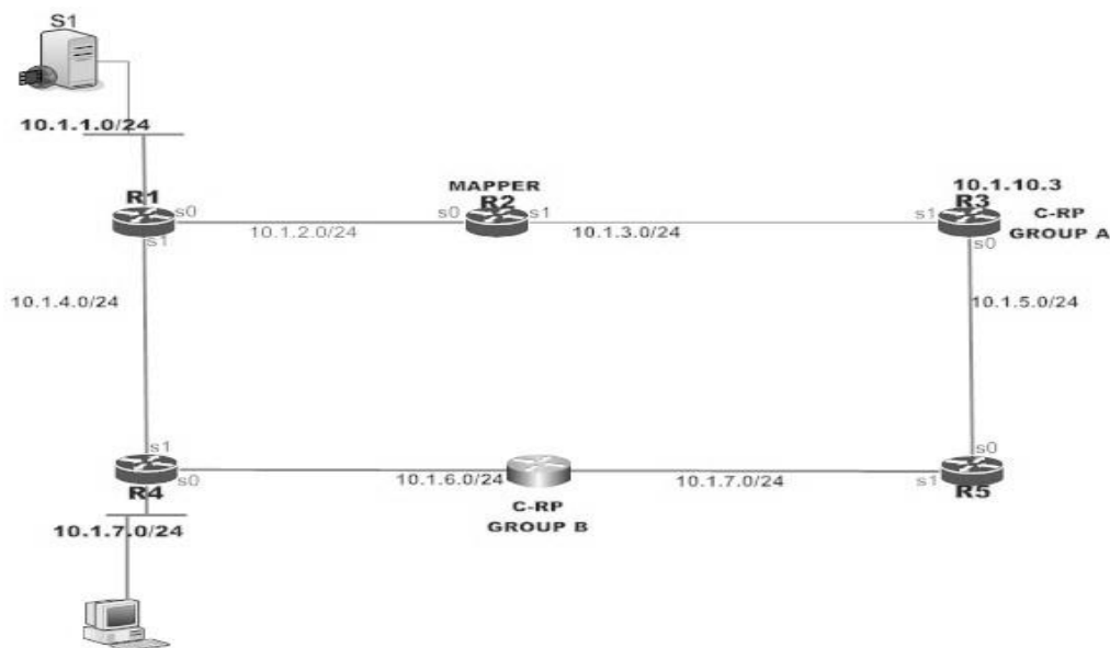
Figure 25 network design with one multicast domain
