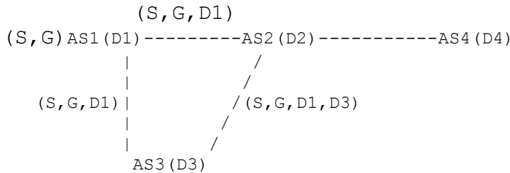
Figure 43 Inter-domain connectivity and RPF check
