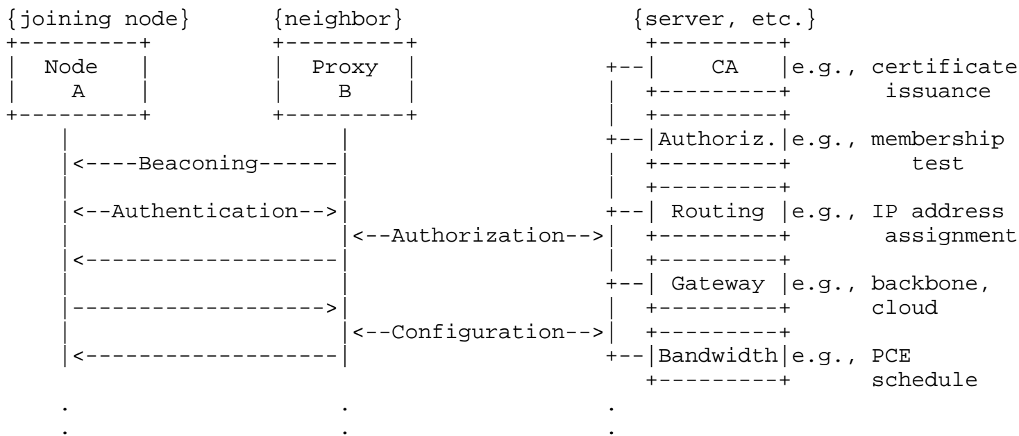
Figure 1: Single-stage authentication/authorization
