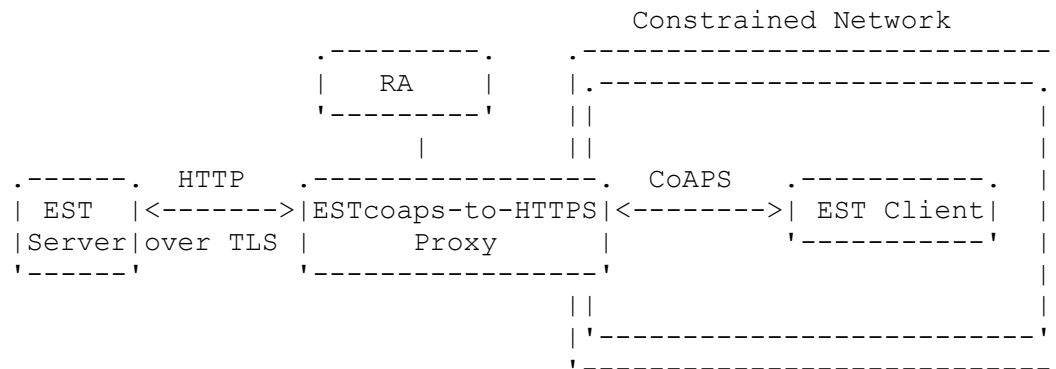
ESTcoaps-to-HTTPS proxy at the CoAP boundary.
