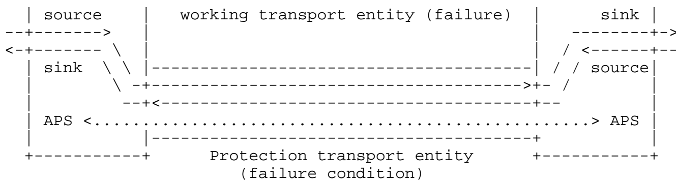
Figure 3: 1:1 bidirectional linear protection switching
