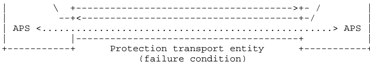
Figure 2: 1+1 bidirectional linear protection switching
