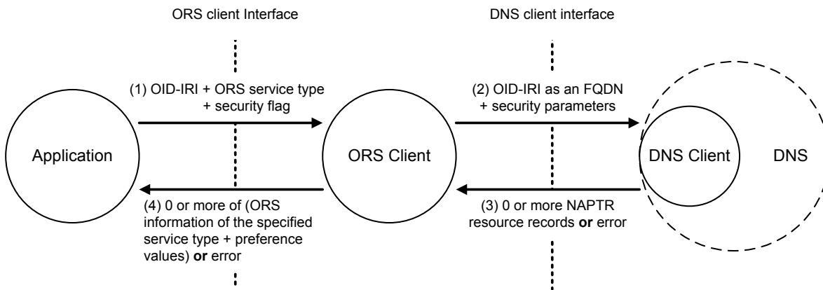
Figure 2 – Components of the general OID resolution system
