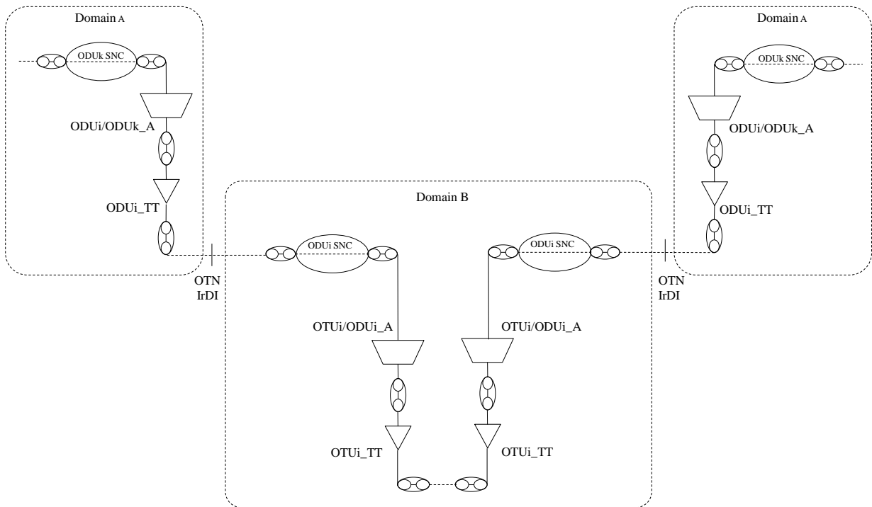
Figure IV.3/G.872 –Multi-domain OTN scenario 3
