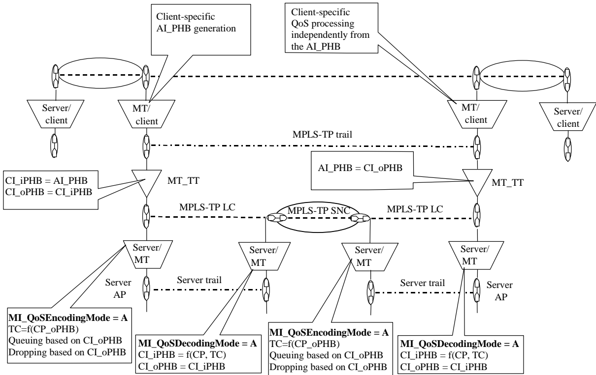
Figure 10-1 – Reference diagram for the short-pipe model
