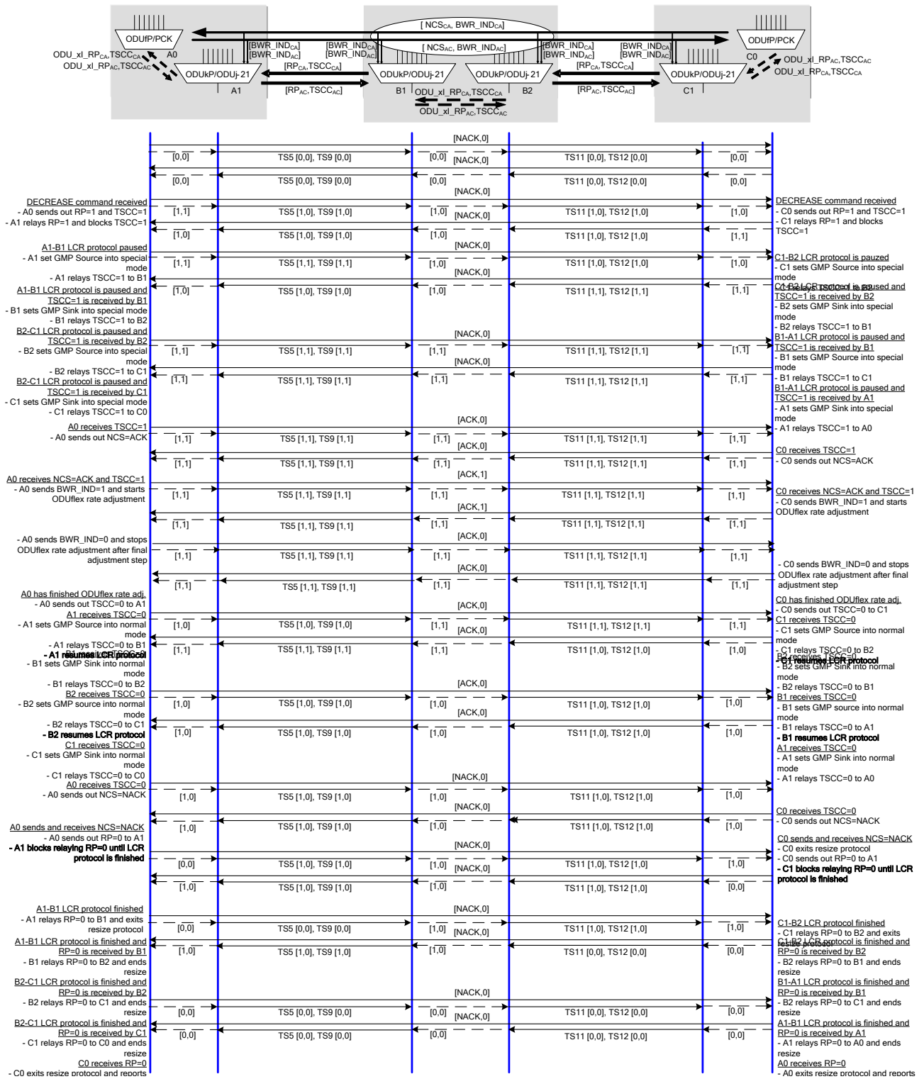
Figure 7-6 – BWR protocol of bandwidth decrease
