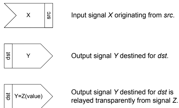
Figure A-2 –SDL legend
