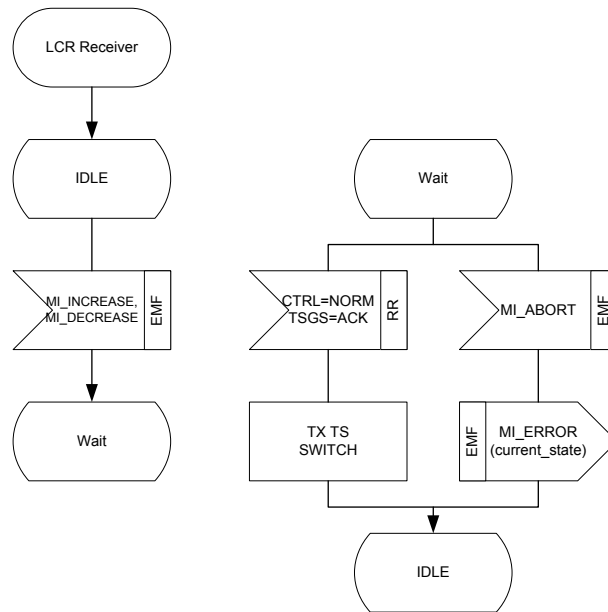
Figure A-4 –SDL diagram for the LCR Receiver
