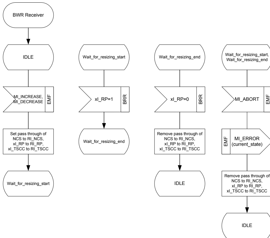
Figure A-6 –SDL diagram for the BWR Receiver
