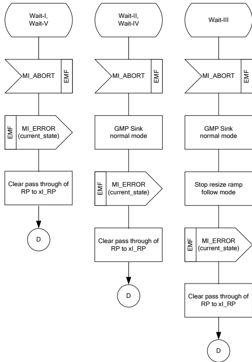
Figure A-8 –SDL diagram for the BWR RELAY Receiver
