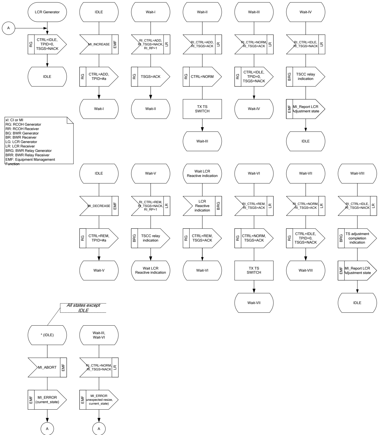
Figure A-3 –SDL diagram for the LCR Generator
