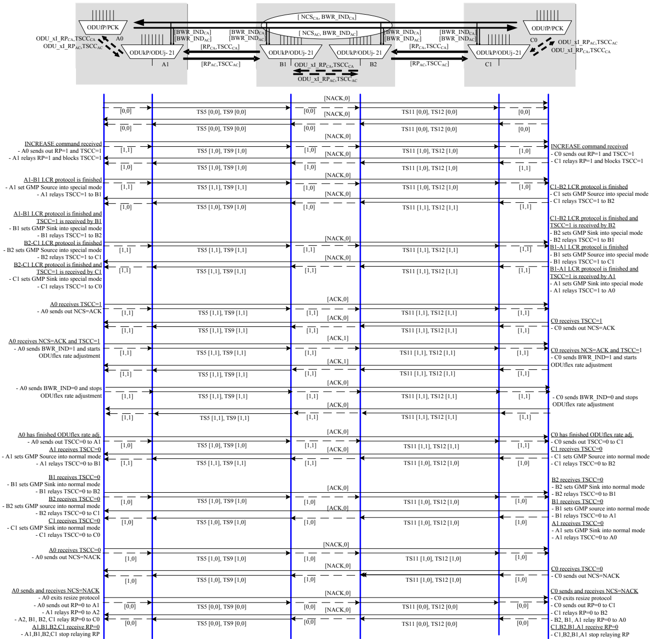
Figure 7-3 – BWR protocol of bandwidth increase
