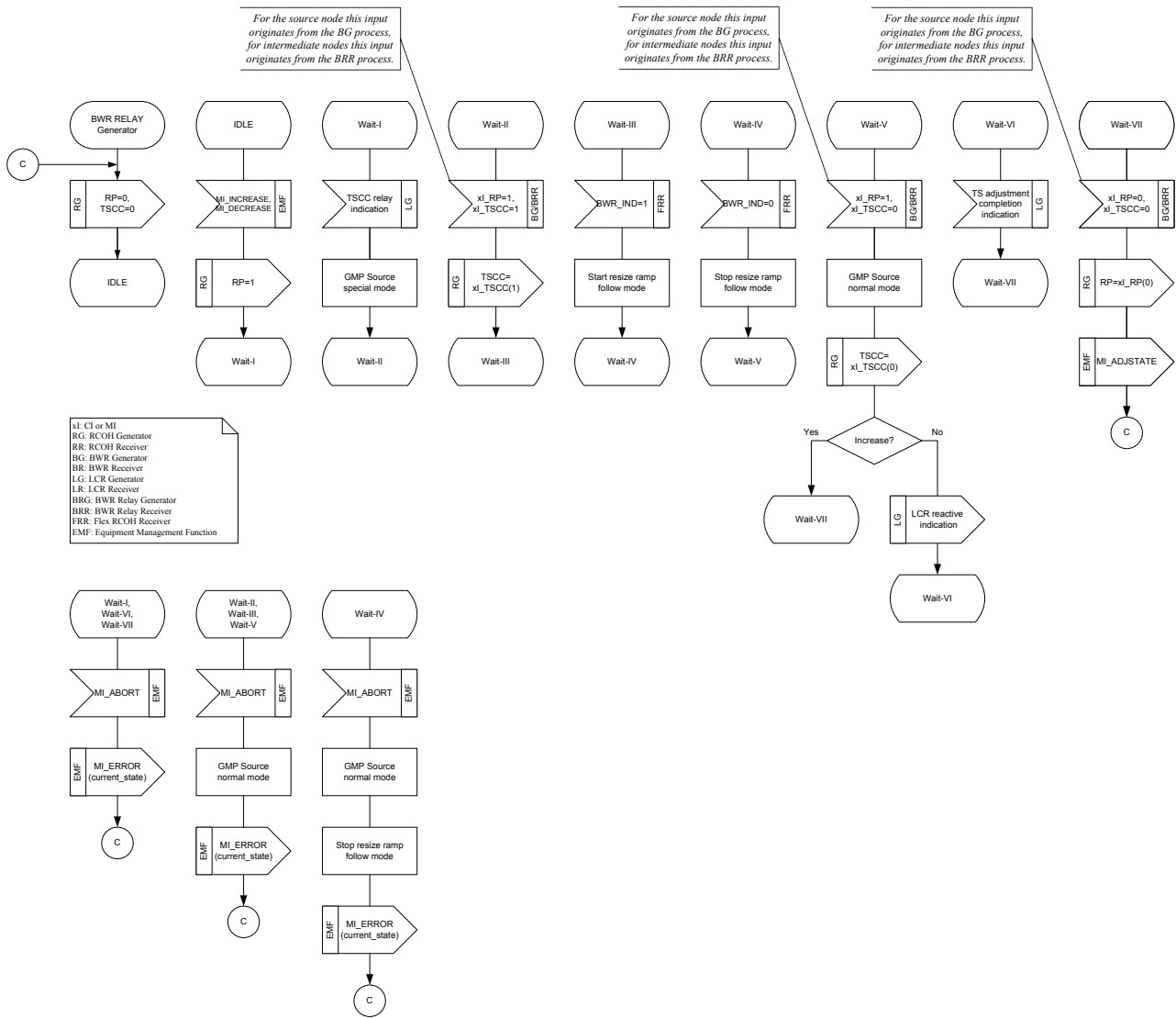
Figure A-7 –SDL diagram for the BWR RELAY Generator
