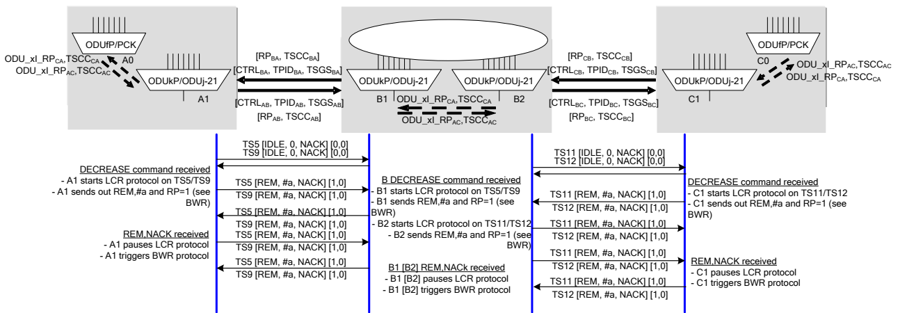
Figure 7-5 –LCR protocol of bandwidth decrease
