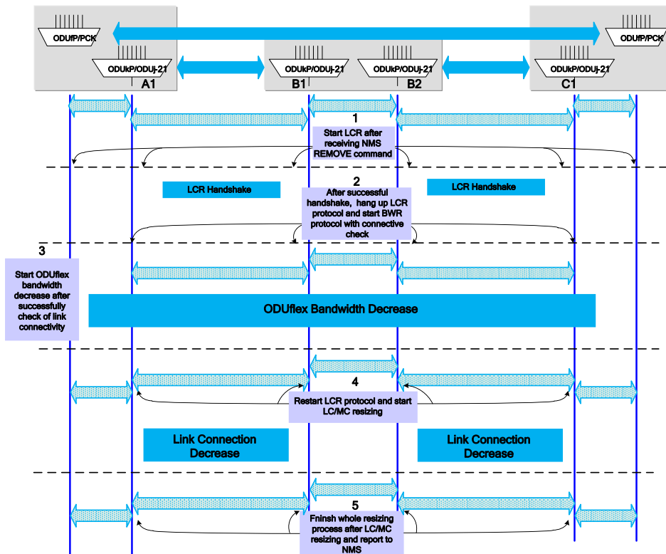
Figure 7-4 – interworking scheme of decreasing case
