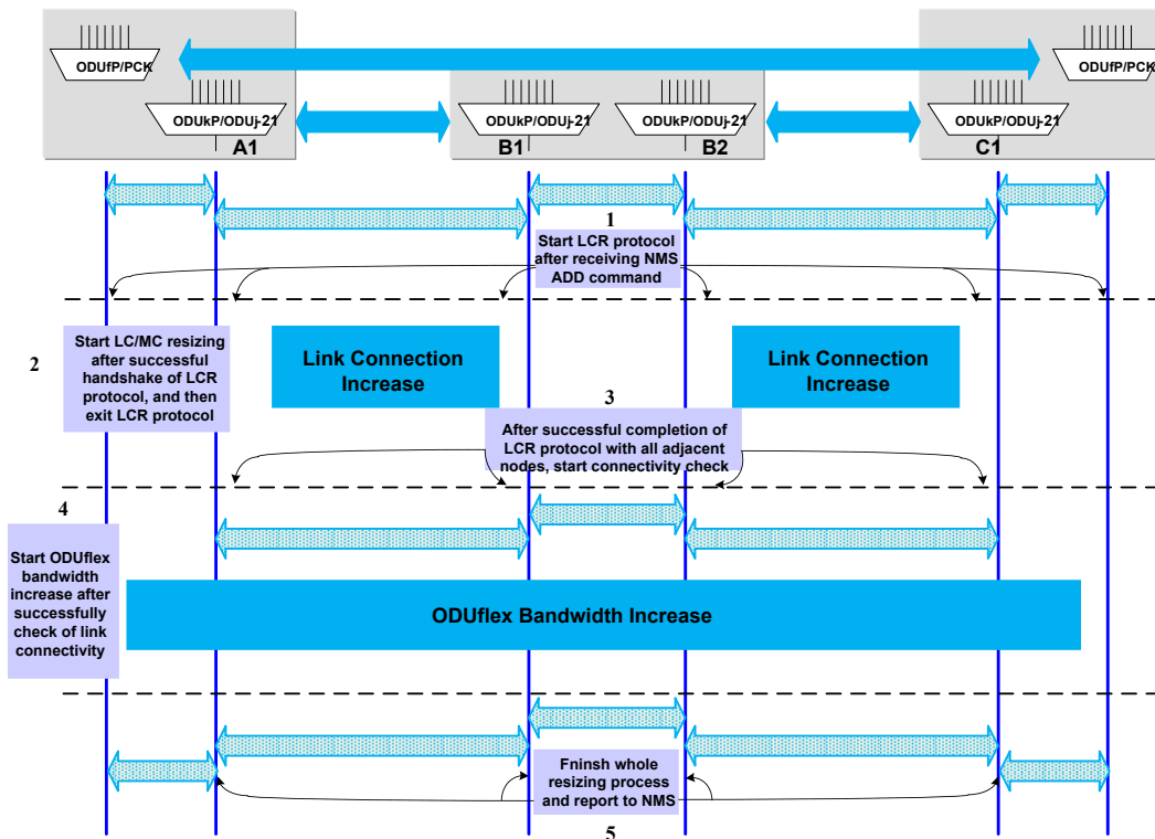
Figure 7-1 – Interworking scheme of increasing case
