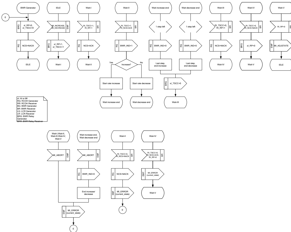
Figure A-5 –SDL diagram for the BWR Generator
