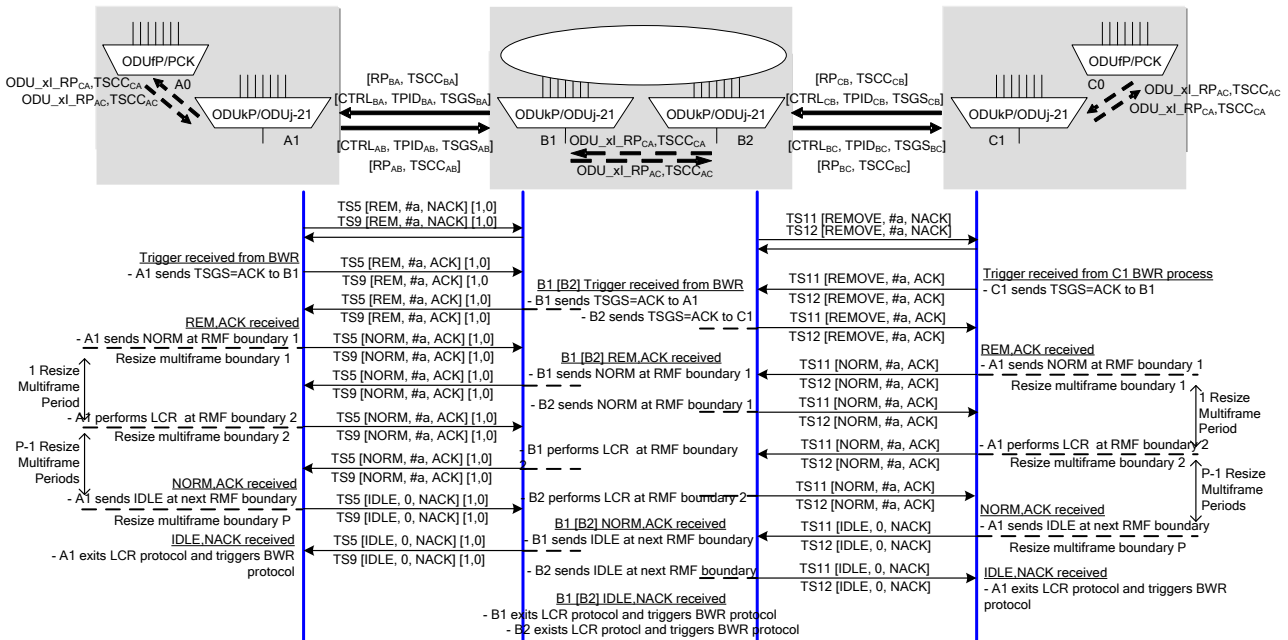
Figure 7-7 – LCR protocol at end of bandwidth decrease
