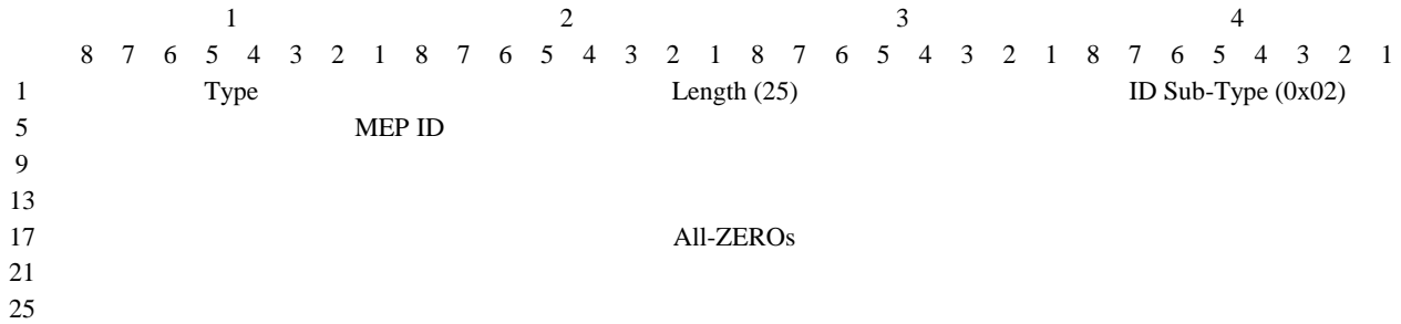
Figure 8-10/G.8113.1 – Target or Replying MEP/MIP ID TLV format for (ICC-based-MEP ID)
