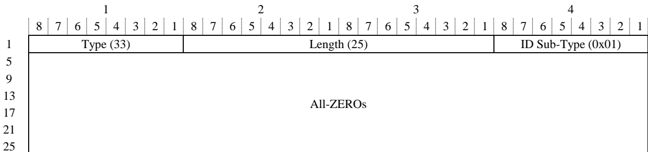
Figure 8-9 /G.8113.1– Target MEP/MIP ID TLV format for Discovery egress MEP/MIP
