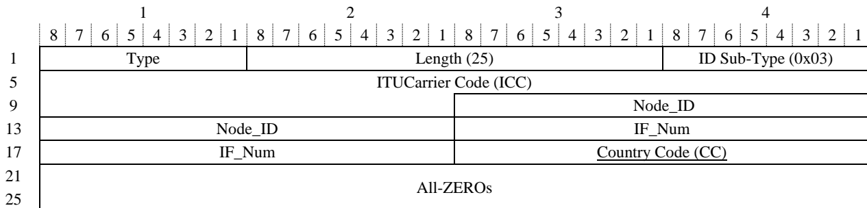
Figure 8-11/G.8113.1 – Target or Replying MEP/MIP ID TLV format for (ICC-based-MIP ID)
