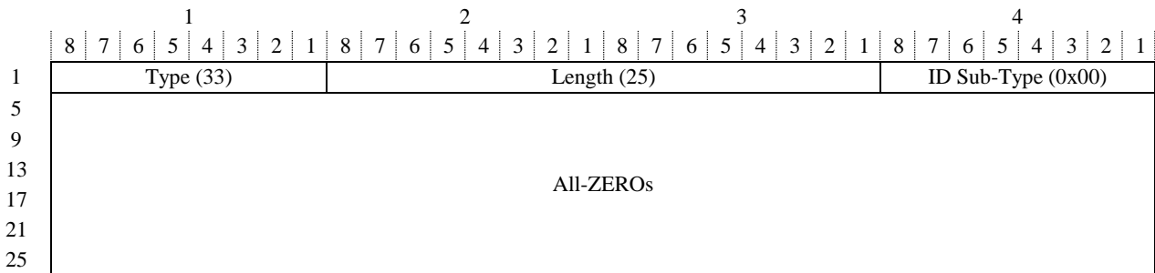
Figure 8-8/G.8113.1 – Target MEP/MIP ID TLV format for Discovery ingress/node MEP/MIP
