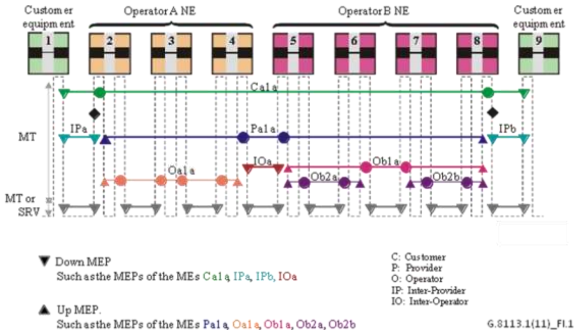
Figure I.1 – Example MEG nesting
