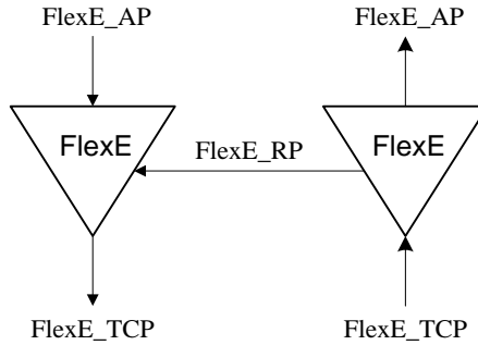
Figure 7-3 – FlexE_TT
