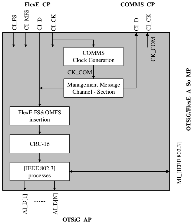
Figure 6-20 – OTSiG/FlexE_A_So processes
