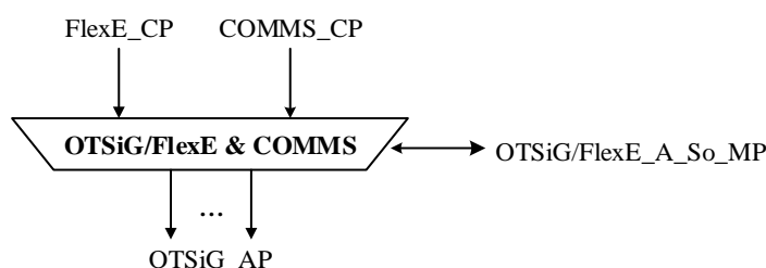
Figure 6-19 OTSiG/FlexE_A_So function
