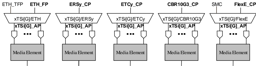
Figure 6-1 – OTSi[G] and ETSi[G] to client adaptation functions
