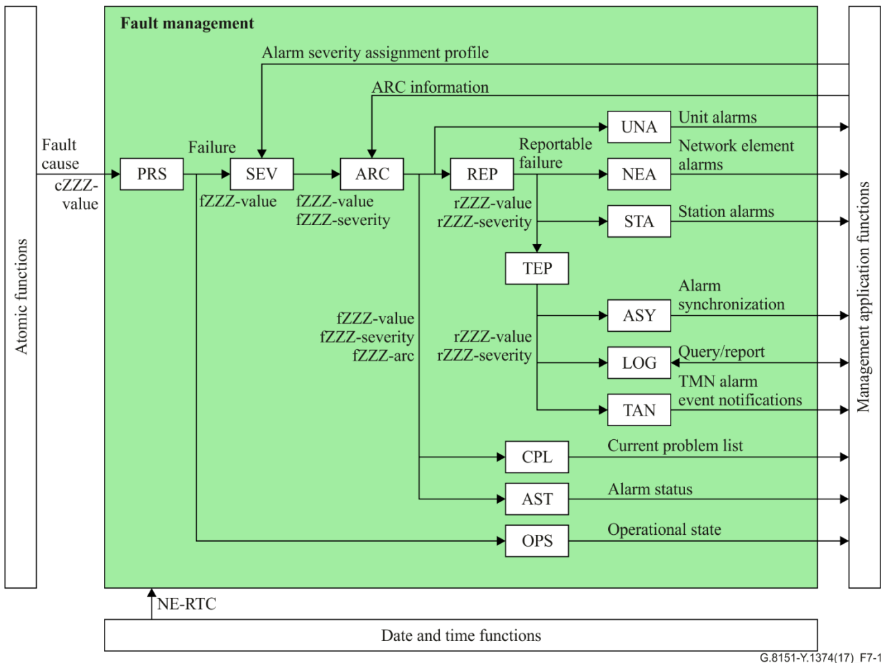
Figure 7-1 – Fault management within the MPLS-TP NEF (from Figure 7-1/G.7710)
