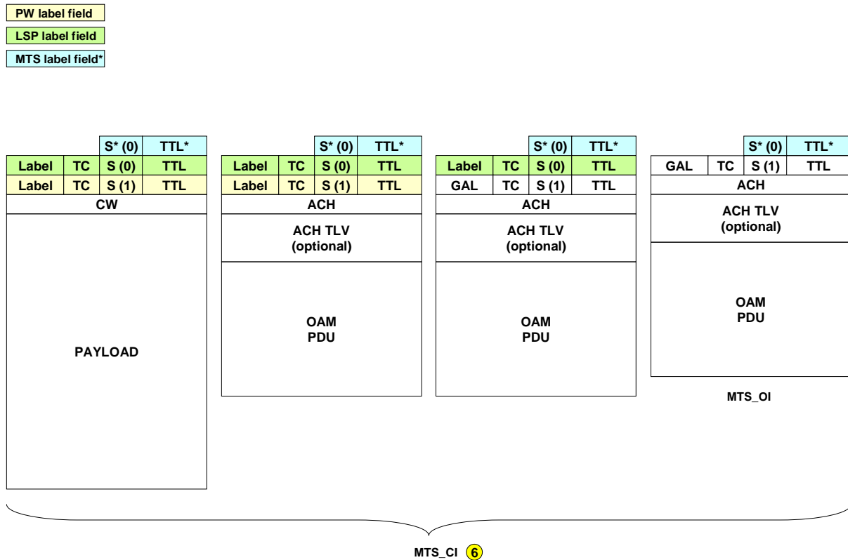
Figure I.5 – MPLS-TP network adapted and characteristic information traffic units (reference point 5)
