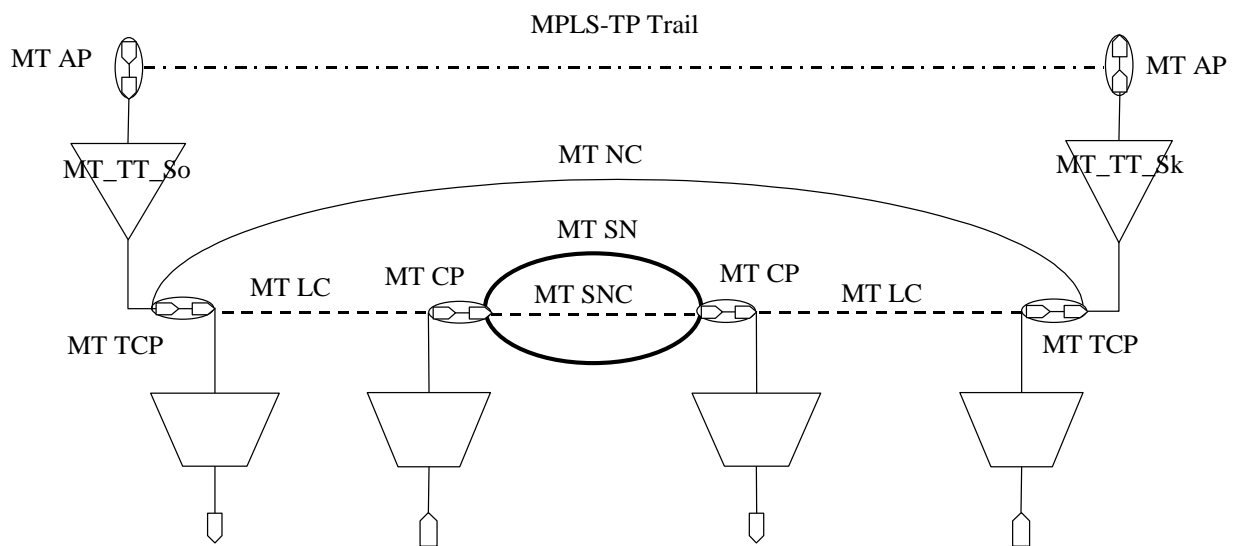
Figure 6-4 – MPLS-TP layer network example
