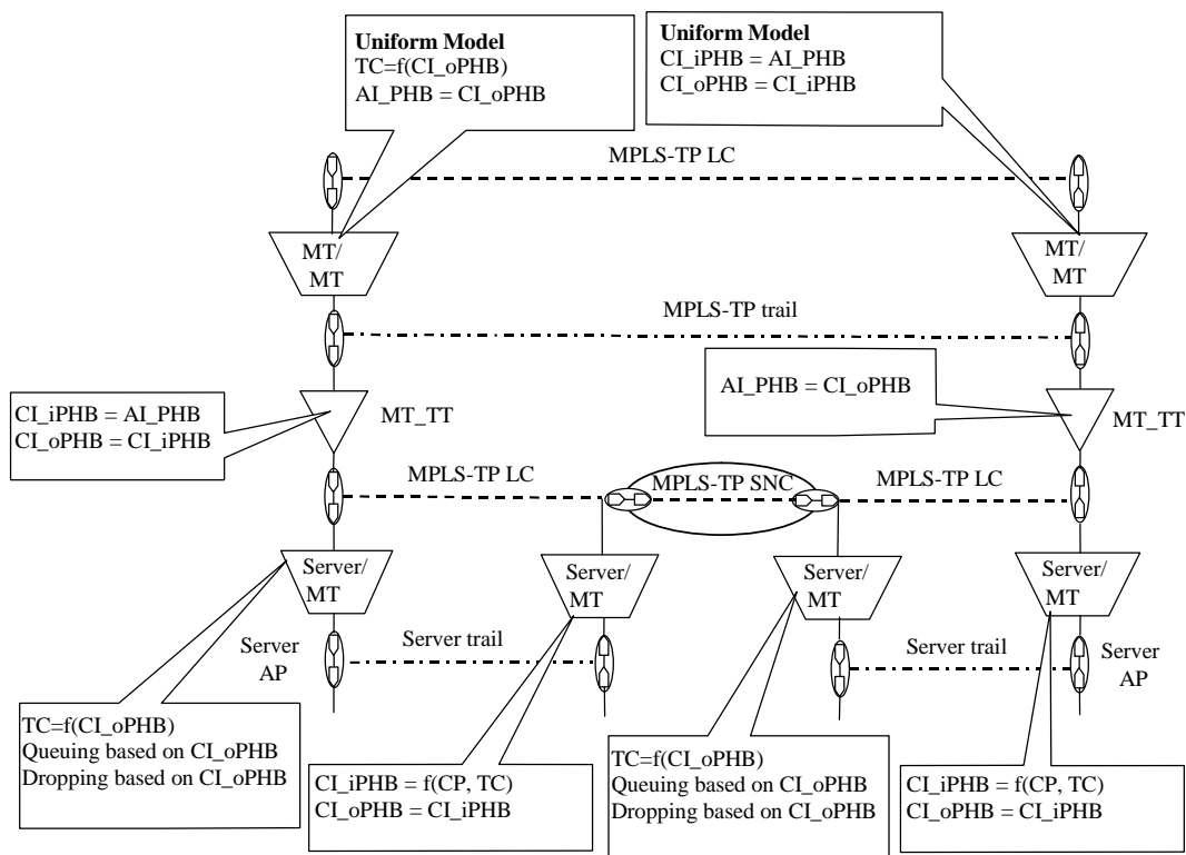
Figure 10-2 – Reference diagram for the uniform model
