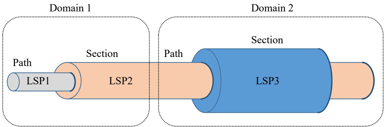
Figure 6-1 – MPLS-TP roles and layers
