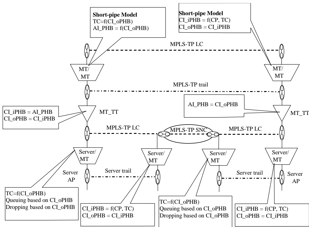
Figure 10-1 – Reference diagram for the short-pipe model
