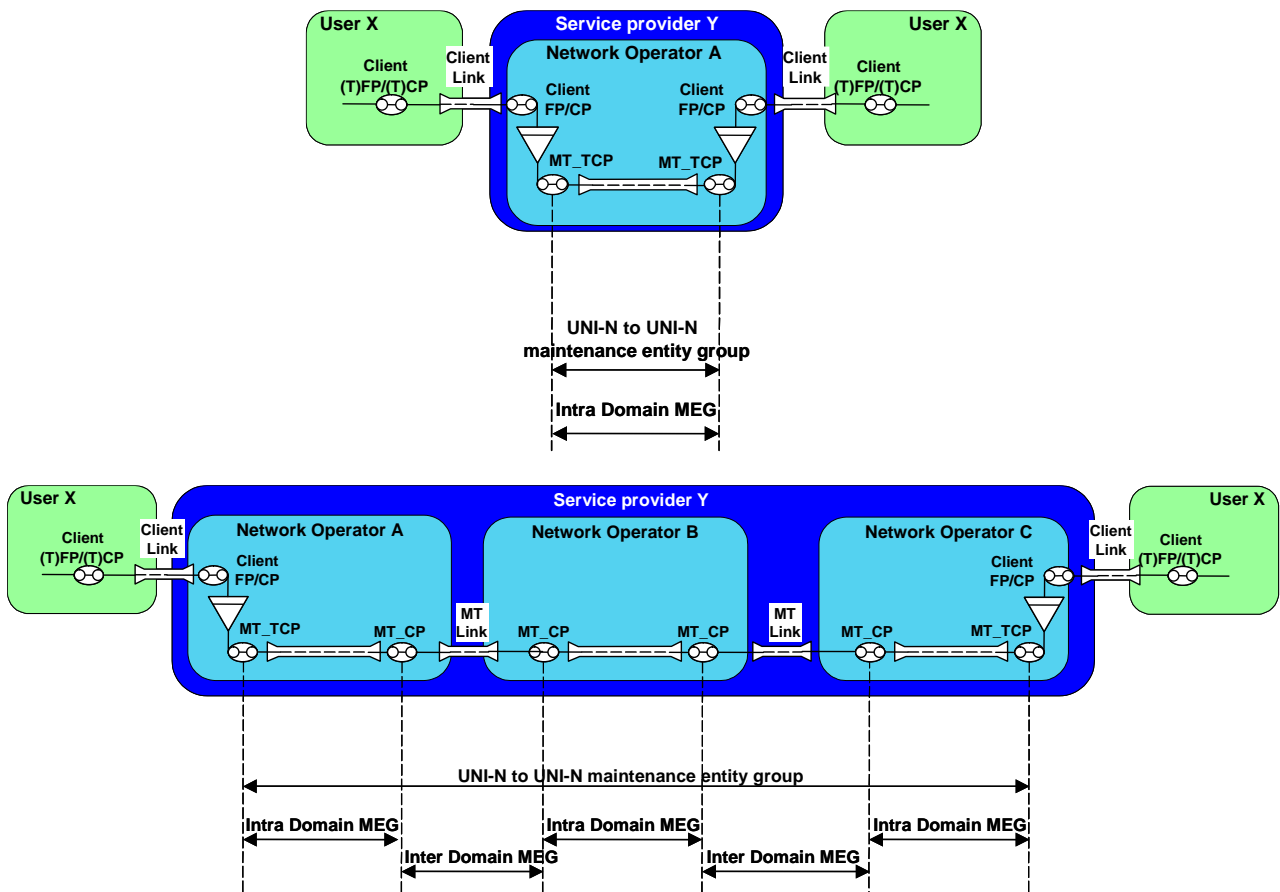
Figure 8-1 – Point-to-point MPLS-TP connection administrative domain associated maintenance entity groups
