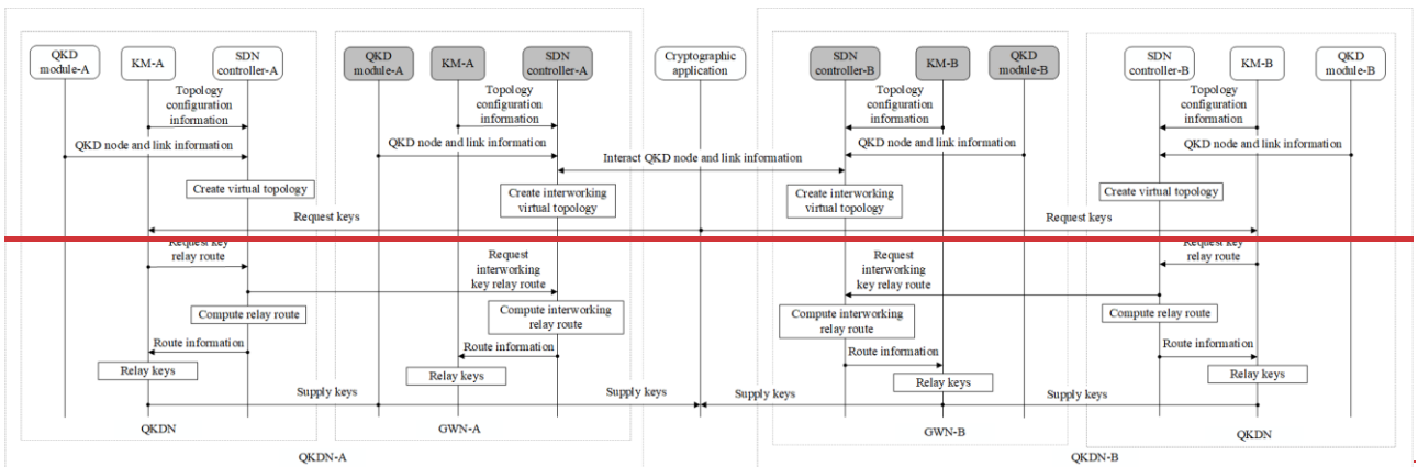
Figure 6—An example of key request, relay and supply phase
