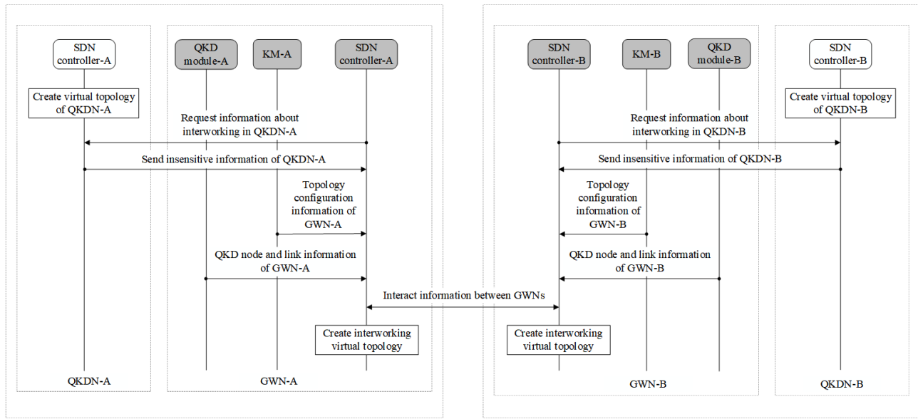
Fig. 1 An example of virtualization phase
