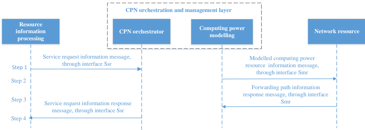
Figure 8-4 Service deployment procedure based on distributed mode
