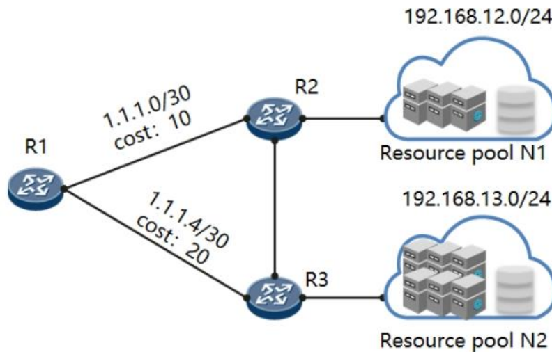
Figure I-1 - An example of network topology
