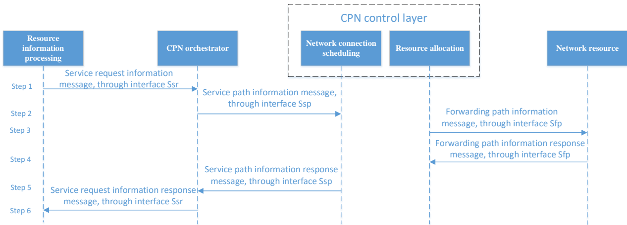
Figure 8-3 Service deployment procedure based on centralized mode
