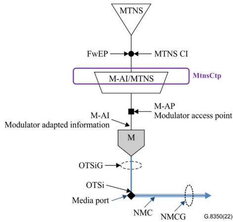
Figure 13-2 – Overview of object class mapping to MTN atomic functions that associated with media layer (Based on Figure 8-1 of [ITU-T G.8310])
