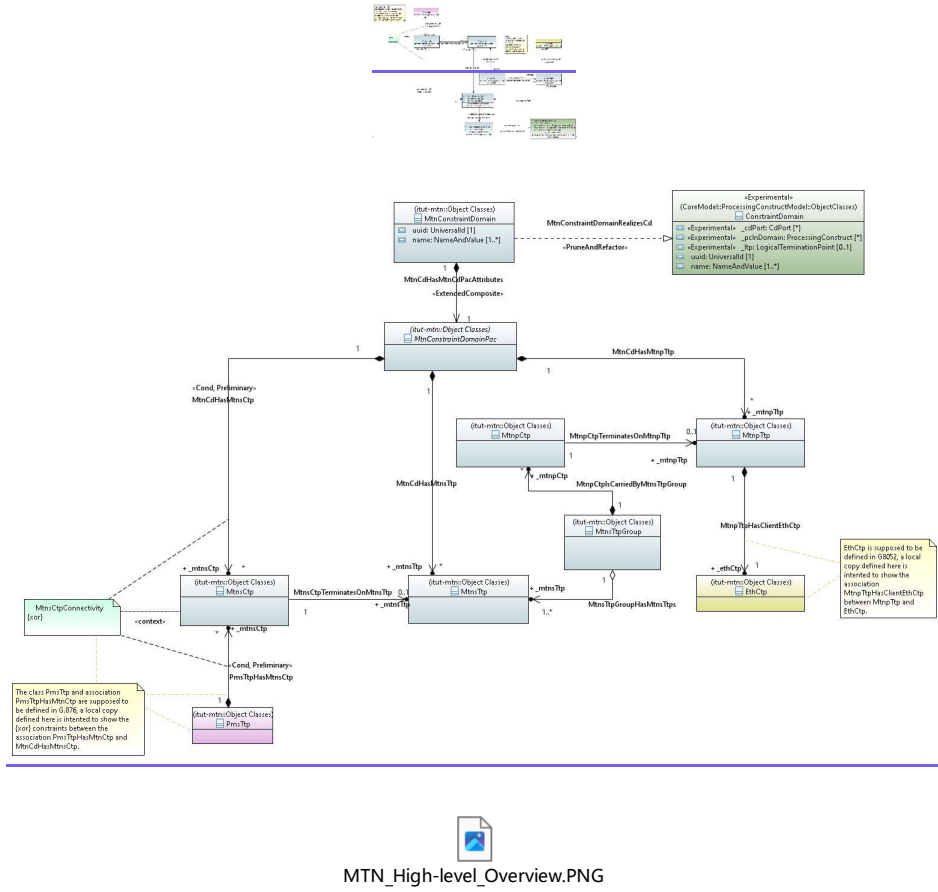
Figure 13-3-4 – MTN model high-level overview
