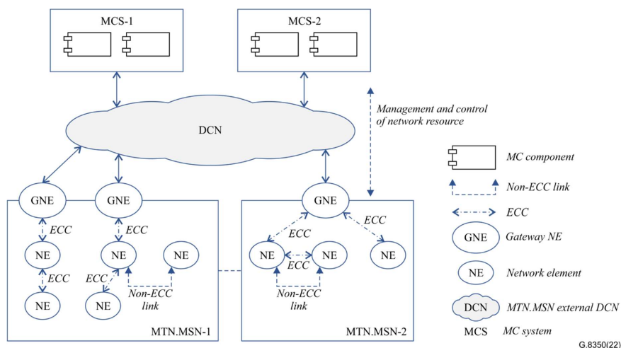
Figure 6-1 – Example of MTN management and control network architecture
