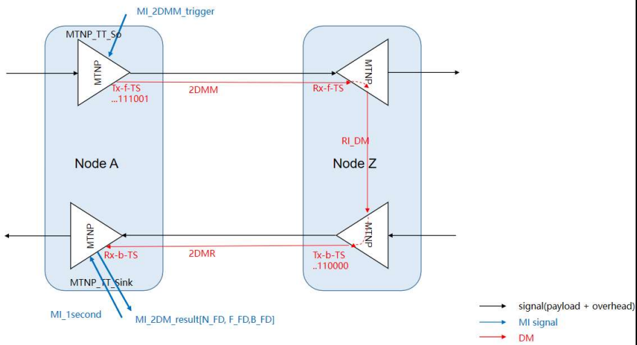
Figure 13-12 single-ended delay measurement function
