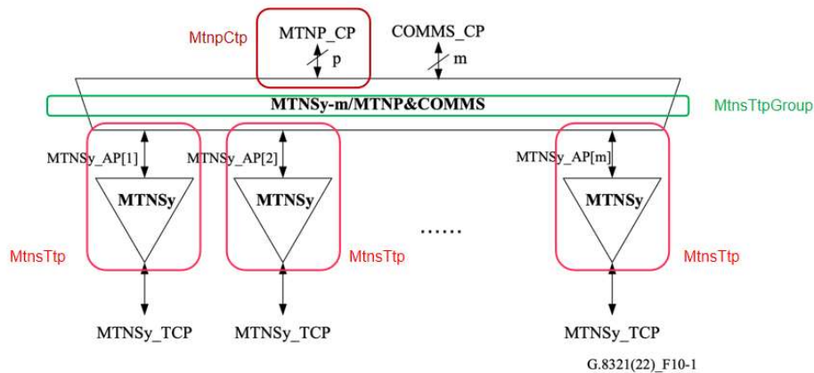
Figure 13-3 Overview of MTNS TTP Group object class mapping to MTN atomic functions (Based on Figure 10-1 of [ITU-T G.8321])
