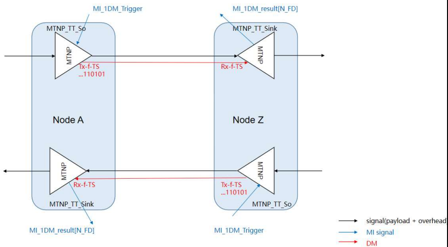
Figure 13-13 dual-ended delay measurement function
