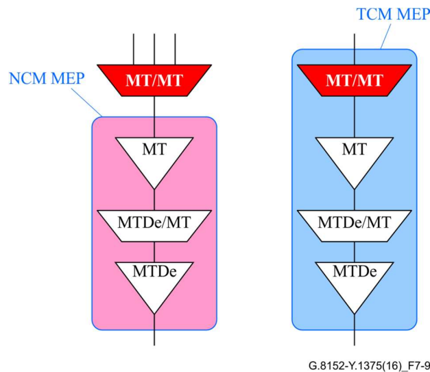
Figure 7-1.D – MPLS-TP multiplexing configuration function
