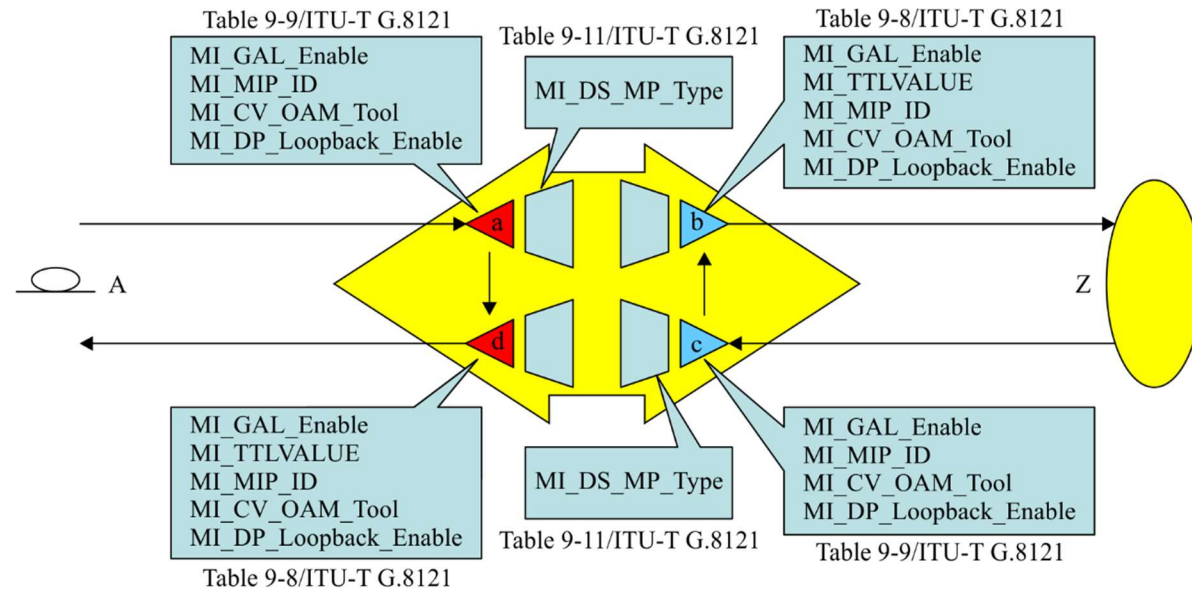
Figure A-6 – MIP configuration parameters
