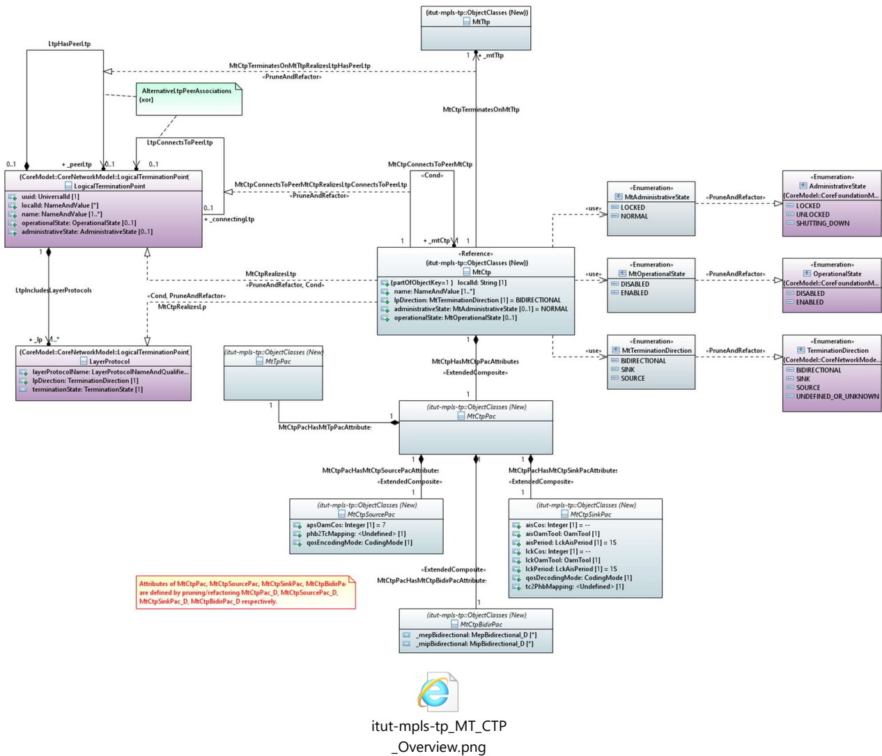
Figure 7-1.A – MPLS-TP CTP Overview
