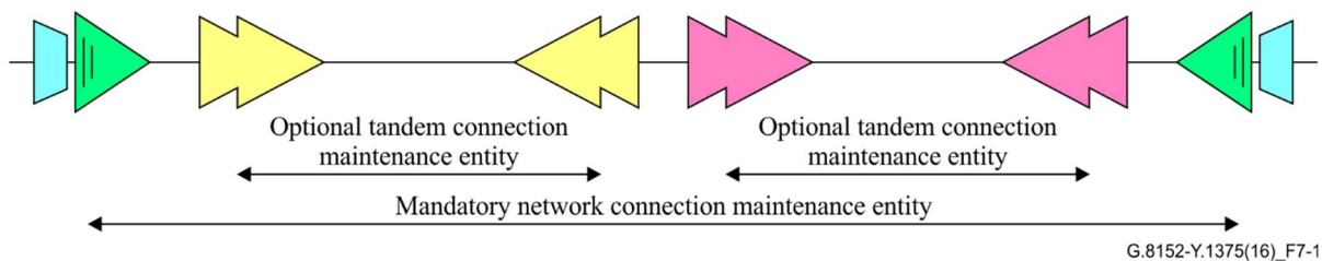
Figure A-1 – Mandatory and optional MEPs
