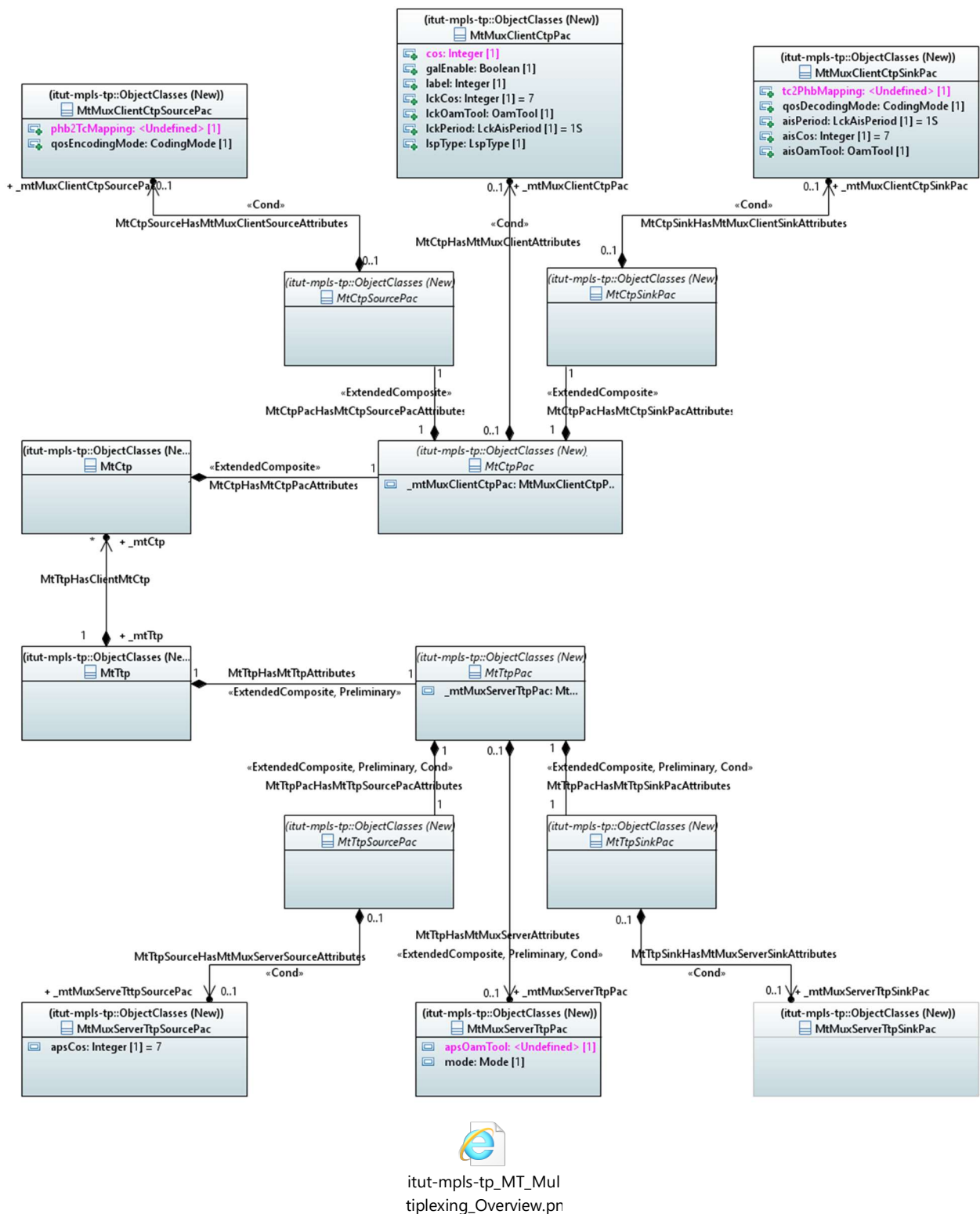
Figure 7-1.E – MPLS-TP multiplexing model overview
