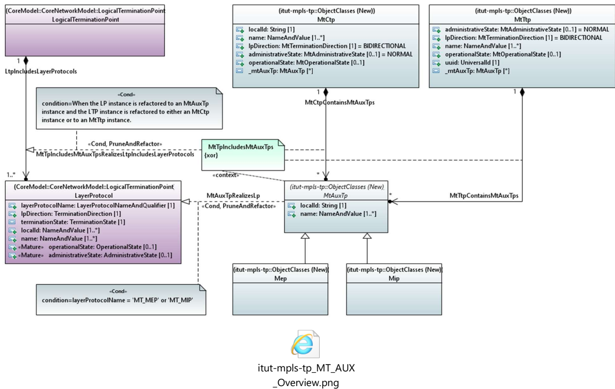
Figure 7-1.F – MPLS-TP auxiliary object classes
