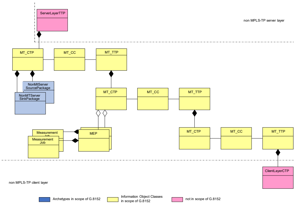
Figure 6-3 – MT layer object instance example with measurement job
