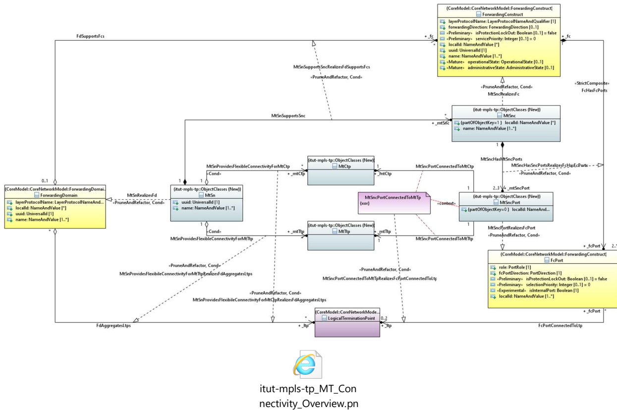
Figure 7-1.C – MPLS-TP connectivity Overview
