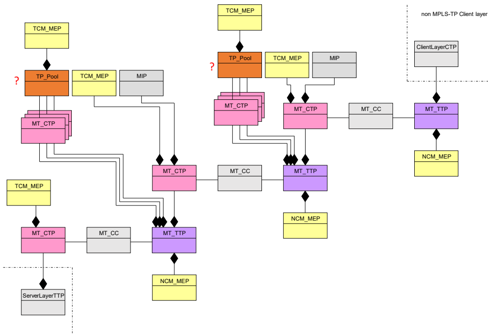
Figure 6-2 – MT object instance example
