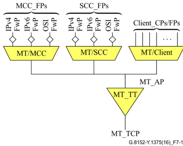
Figure A-11 – MT/SCC_A function, MT/MCC_A function, and MT/client_A function (Copy from Figure 10-5 [ITU-T G.8121])
