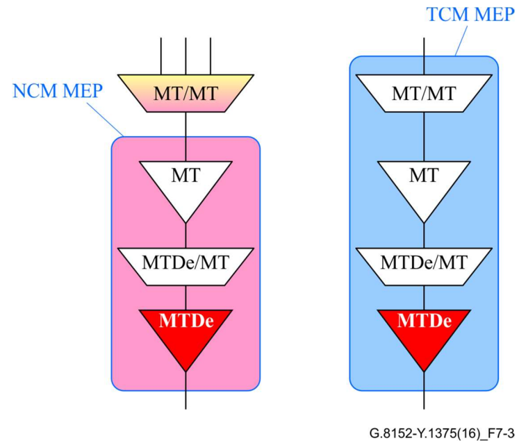
Figure A-3 – MEP on-demand diagnostic function
