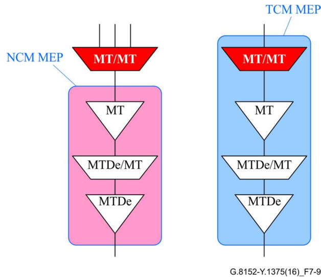
Figure A-9 – MPLS-TP multiplexing configuration function
