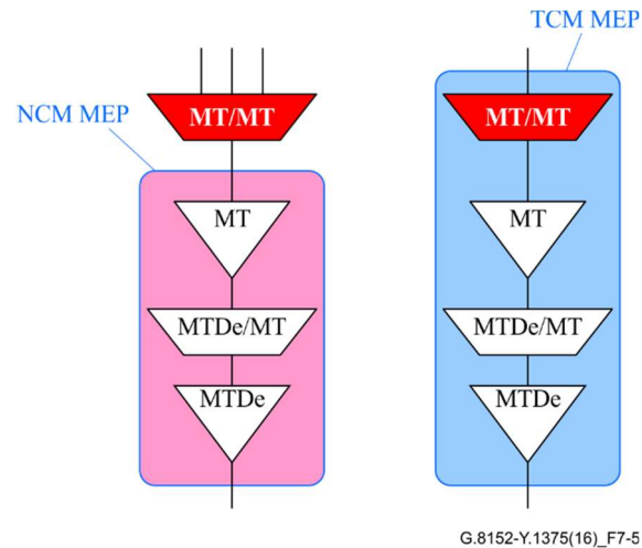
Figure A-5 – MEP configuration function
