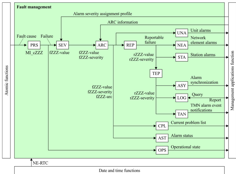
Figure 7-1 – Fault management within the optical transport network network element function (Figure 7 of [ITU-T G.7710])
