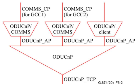
b) For ODUCnP access point (AP)
