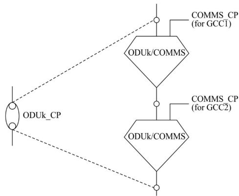
a) ODUk_CP expansion for COMMS access
