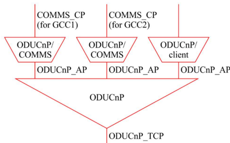
b) ODUcn_CP expansion for COMMS access
