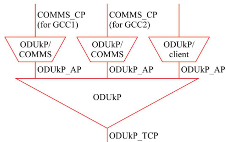
a) For ODUkP access point (AP)
