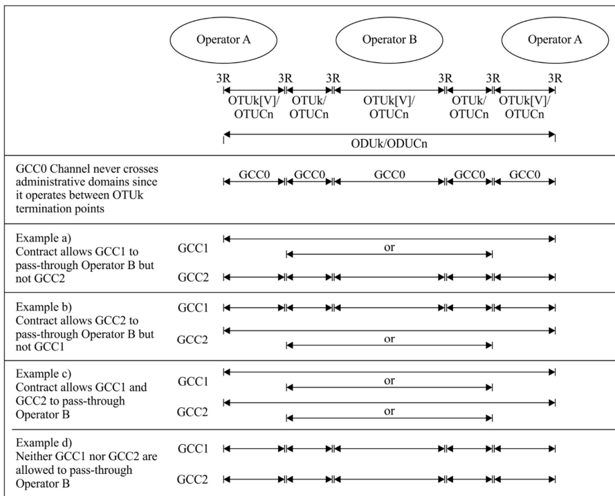
Figure 6-1 – GCC contract scenarios OTUk[V]: OTUk or OTUkV
