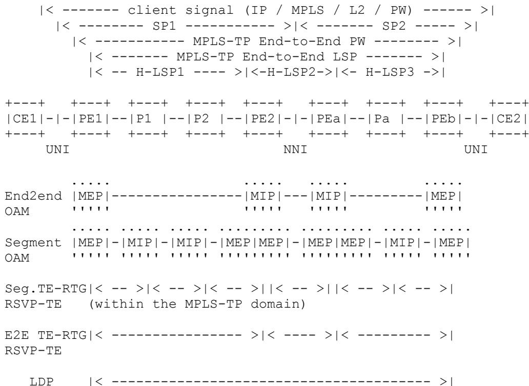
Figure 2. [M32]MPLS-TP Control Plane Reference Model with OAM
