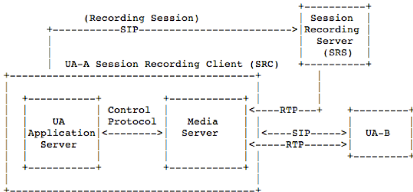
Figure 4: Example of Session Recording Client decomposition
