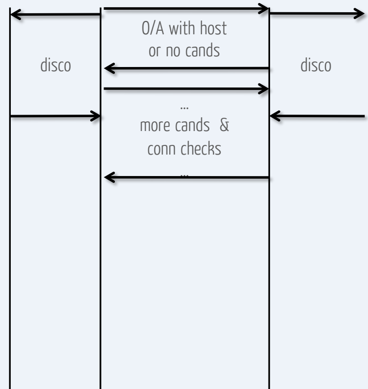
Trickle ICE
