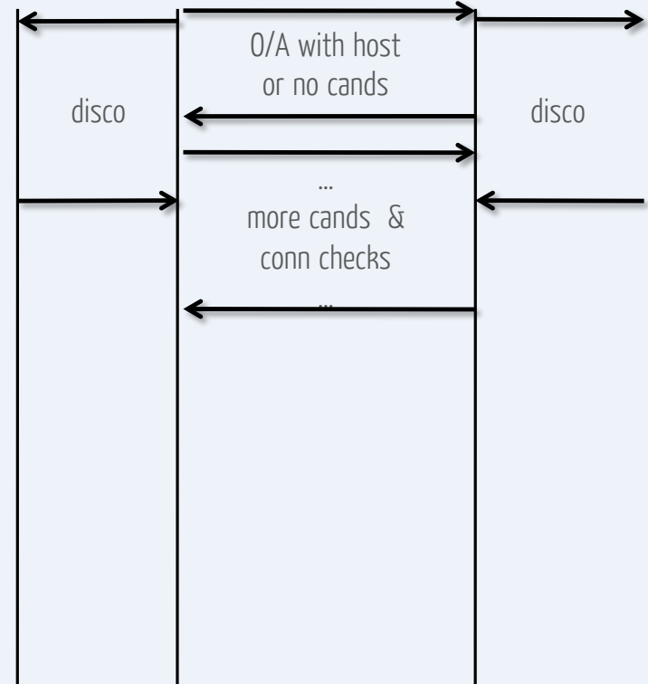
Trickle ICE
